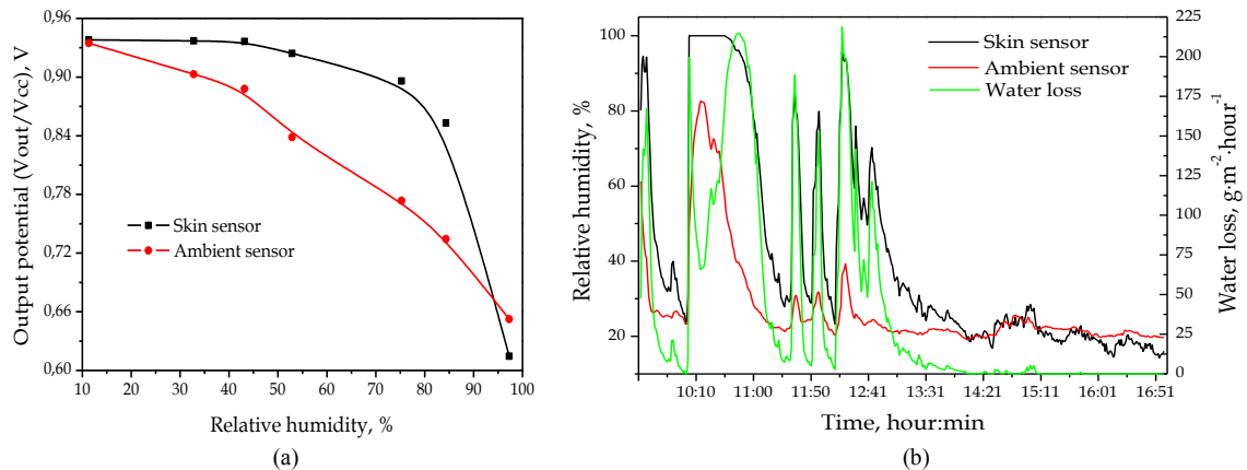
Fig. 4. (a) relative humidity sensors calibration plot; (b) portable perspiration system testing diagram
