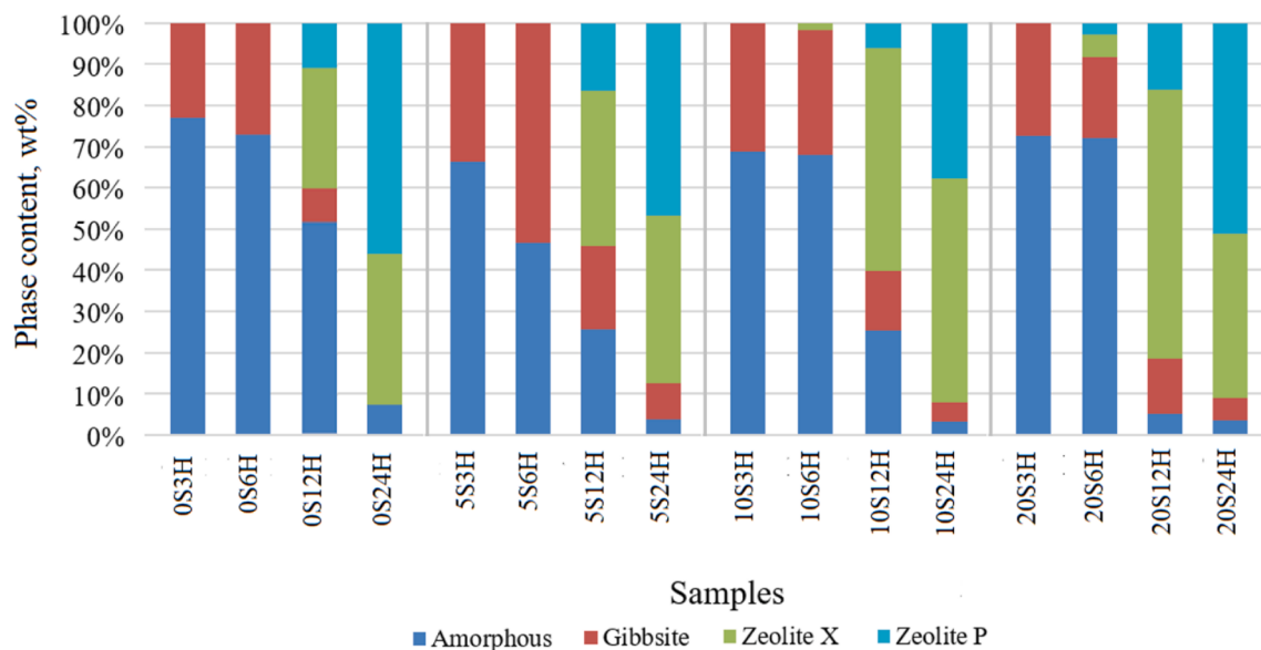
Fig. 4. The phase composition of synthesis products.
