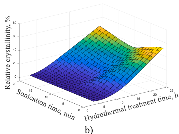
Fig. 5. Crystallization graphics of conversion of silica by-product to Na-X zeolite (a) and Na-P zeolite (b) using ultrasonic-assisted hydrothermal treatment.
