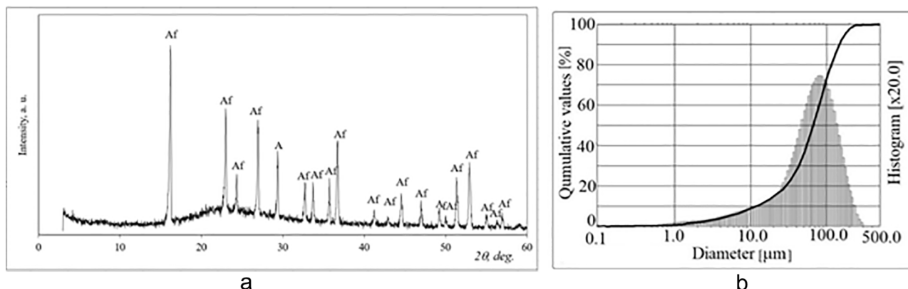
Fig. 1. The X-ray diffraction pattern (a) and particle size distributions (b) of silica by-product. Note: Af is aluminium fluoride hydrate \text{AlF}_3 \cdot 3.5\text{H}_2\text{O} (35–827).
