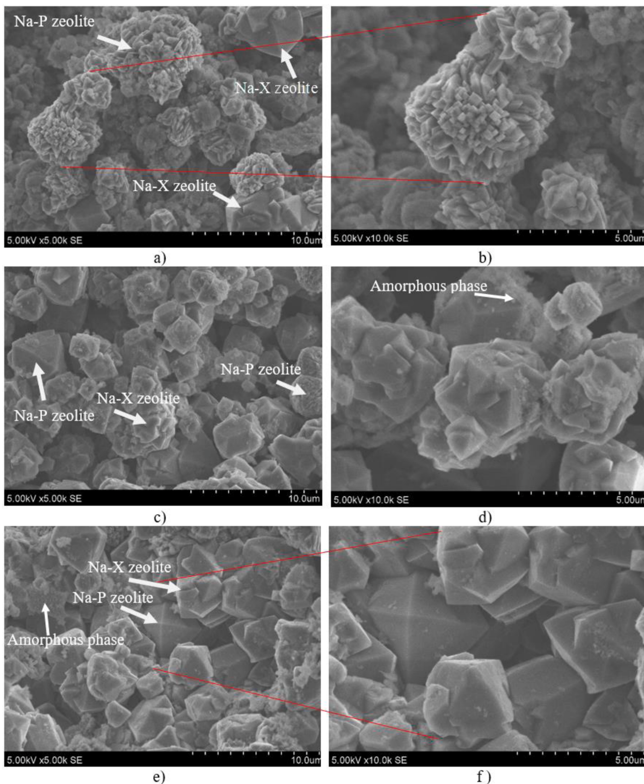
Fig. 7. Microstructure of synthesized products at different magnification (scale 5 µm and 10 µm). Notes: a, b – 0S24H; c, d – 20S12H e, f – 20S24H.
