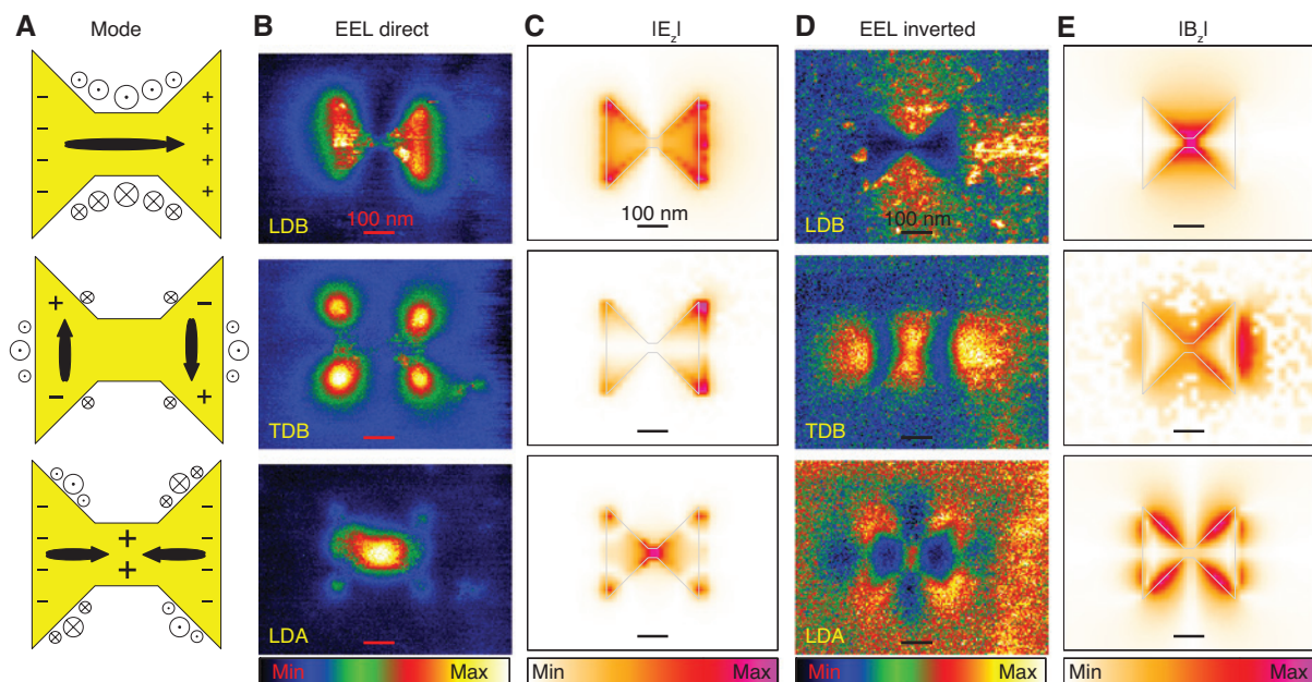
Figure 6: Experimental EEL maps and calculated fields for the LDB (1st row), TDB (2nd row), and LDA (3rd row) modes. (A) Schematic representation of the mode in the diabolo antenna. The black arrow depicts the current with the thicker middle part representing the current antinode and the thinner border parts representing the current node. Magnetic field in the plane of the antenna is schematically represented by \odot (outward field) and \otimes (inward field) symbols with the size corresponding to the magnitude of the field. The node of current corresponds to the accumulation of the charge represented by + and - symbols. (B) Experimental loss intensity distribution. (C) Calculated out-of-plane electric field. (D) Experimental loss intensity distribution for Babinet-complementary antenna (inverted diabolo). (E) Calculated out-of-plane magnetic field. The length of the scale bars is 100 nm.
