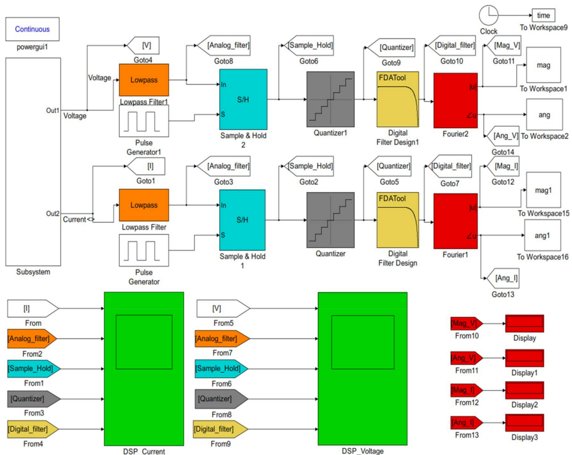
Figure 2. Model for current/voltage signal processing (DSP).
