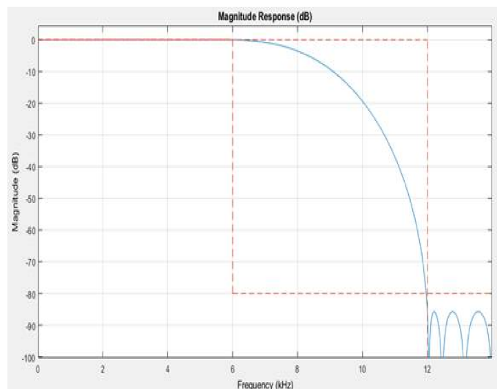
Figure 3. Low pass filter block characteristics.
