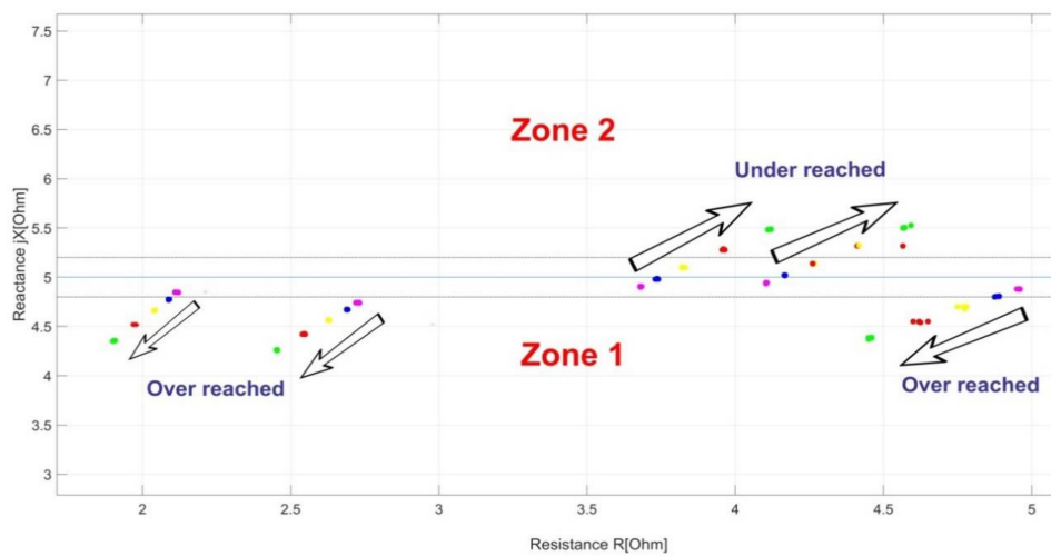
Figure 10. Quadrilateral characteristic and measured fault impedance locus.
