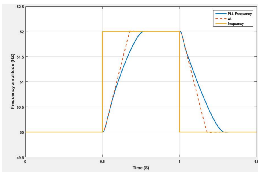
Figure 5. Frequency variation measurements between 50 and 52 Hz.
