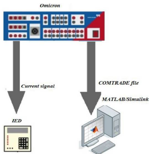
Figure 1. The test structure.
