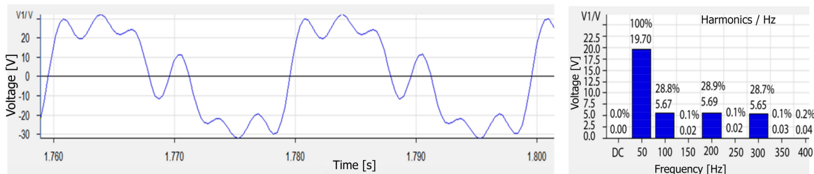
Figure 8. Decomposed voltage waveform with Fourier transform/Matlab window.
