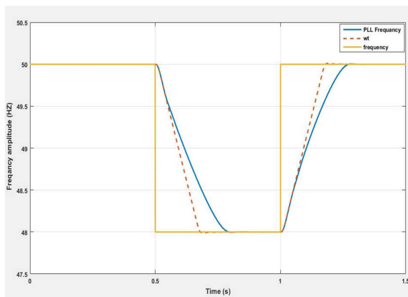
Figure 6. Frequency variation measurements between 48 and 50 Hz.
