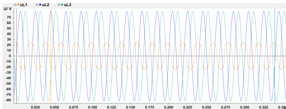
Figure 11. Voltage waveforms during single-phase fault (IED).
