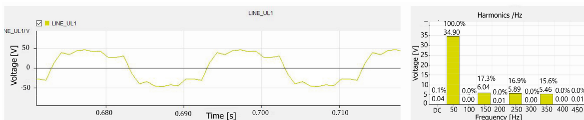
Figure 9. Decomposed voltage waveform with Fourier transform/Matlab window.
