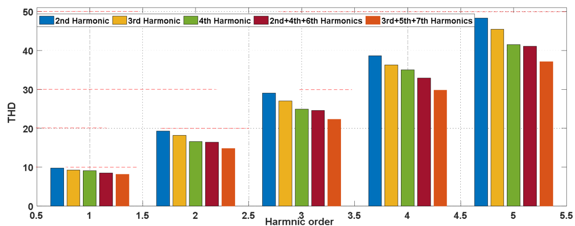
Figure 14. Commercial relay measurement of THD.
