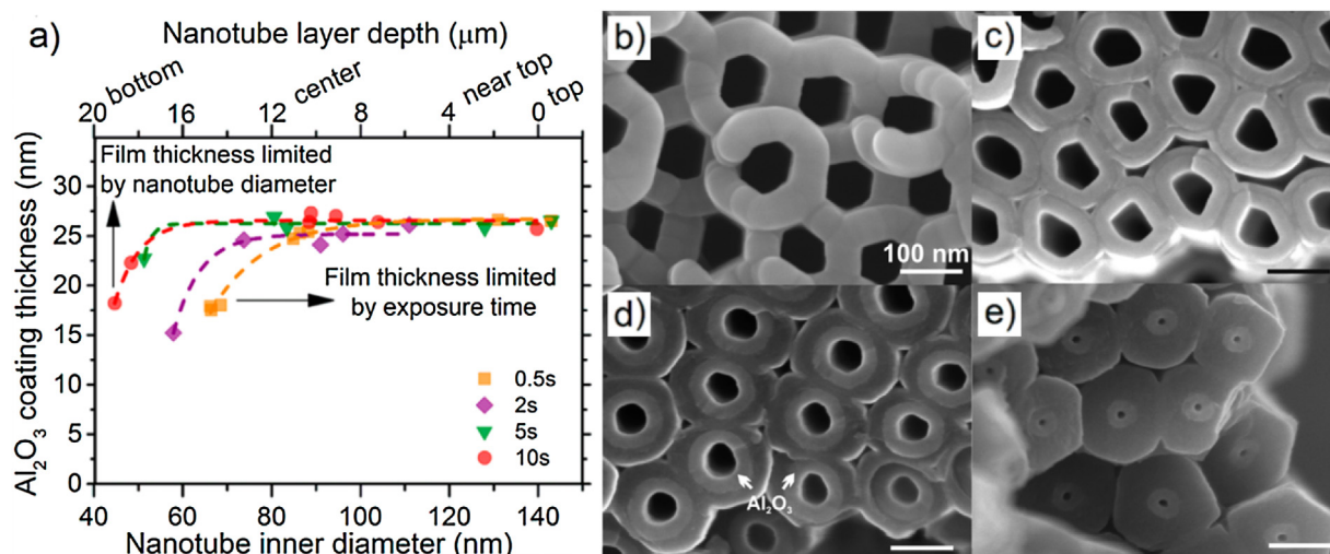
Fig. 5. ALD \text{Al}_2\text{O}_3 coating of TNT layers with aspect ratio of 180: (a) Influence of exposure time of TMA precursor during one ALD cycle on uniformity of thickness of \text{Al}_2\text{O}_3 coating within TNT layer; (b–e) Illustration of uniform thickness of \text{Al}_2\text{O}_3 coating for 5 s TMA exposure time as revealed by SEM inspection through four different depth levels – top, near-top, middle, and bottom, respectively. Reproduced from [118].
