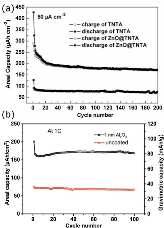
Fig. 12. (a) Charge/discharge capacity of bare and ALD ZnO coated TNT layer as a function of charge/discharge cycles, reproduced from [200]. (b) Improved charge capacity of ALD \text{Al}_2\text{O}_3 coated TNT layer as compared with uncoated TNT layers throughout multiple charge/discharge cycles, reproduced from [201].
