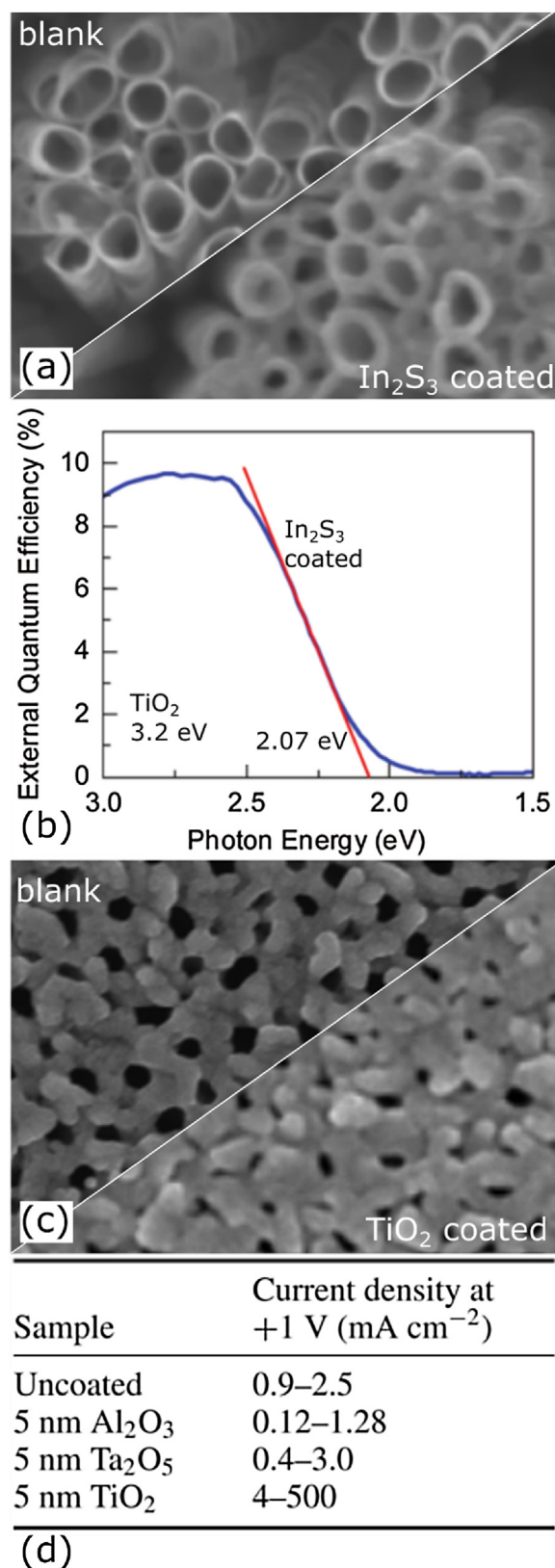
Fig. 4. Pioneering ALD coatings of TNT layers. (a) The \text{In}_2\text{S}_3 coating of TNT layers and (b) corresponding quantum efficiency. (c) The \text{TiO}_2 coated TNT layer and (d) the current density through the TNT layer modified by various metal oxide coatings. (a) and (b) were reproduced from [115] and (c) and (d) were reproduced from [116].
