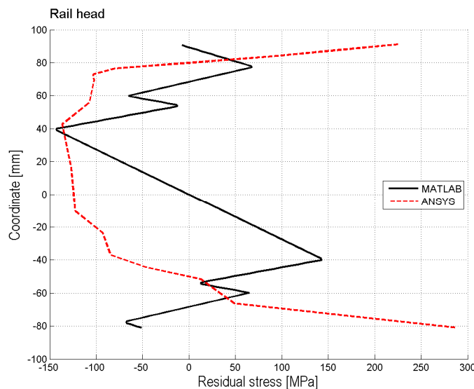
Fig. 4: Residual stress after straightening.
