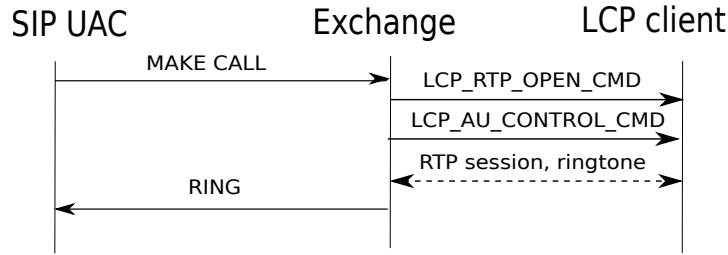
Figure 2.1: Message sequence chart of LCPCPv1 behaviour
