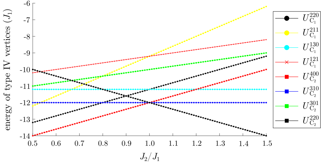
Fig. 4.15: Computed energy spectrum for type IV _{C_1} and type IV _{C_2} vertices. The energy of a vertex type depends on the J_2/J_1 ratio. The J_1 value affects the mutual hierarchy of type IV _{C_1} and type IV _{C_2} . For this computation, the J_1 value is set to J_1 = 0.9J_1 .
