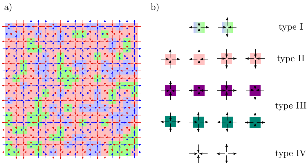
Fig. 2.3: a) Example of a typical spin-liquid state composed of a mixture of type I and type II vertices. In all spin configurations, the colour of spins (arrows) depends on the orientation by the next convention. Horizontal spins pointing to the right (resp. to the left) are blue (resp. red). Vertical spins pointing upward (resp. downward) are blue (resp. red). This convention helps to directly observe line ordering (typical example can be seen in figure 3.7b). Type I vertices are portrayed by light green and blue squares. Regions, where type I vertices are connected together, are then more recognisable. Type II which separates blue and green islands of type I is portrayed by light red squares. Spin configuration was obtained by Monte Carlo simulation. b) Overview of all 16 possible vertex configurations. Type I and type II are the only types that fulfil the so-called ice rule . Type III and type IV are excitations of the system and violate the ice rule. The spin configuration is adapted from [34].
