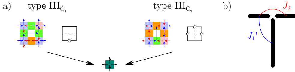
Fig. 4.11: a) Examples of two spin configurations in the shakti lattice for type III_{C_1} and type III_{C_2} . Even with different spin configurations in the shakti lattice, the plaquette is projected to an identical type III vertex. b) Interactions between first ( J_1 ) and second ( J_2 ) neighbours at the T junction.
