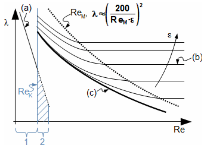
Obr. 3.2 — Moodyho diagram [28]
