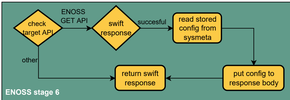
Figure 5.5: ENOSS middleware stages 6 - Reading stored configuration.
