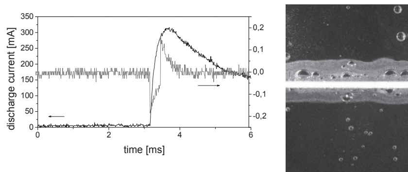
Figure 4. Experiment with the diaphragm with the smaller orifice (diameter of 0.3 mm) and thickness of 1.0 mm. Camera closing by a current impulse (left). Photography exposure time of 0.5 ms (right).
