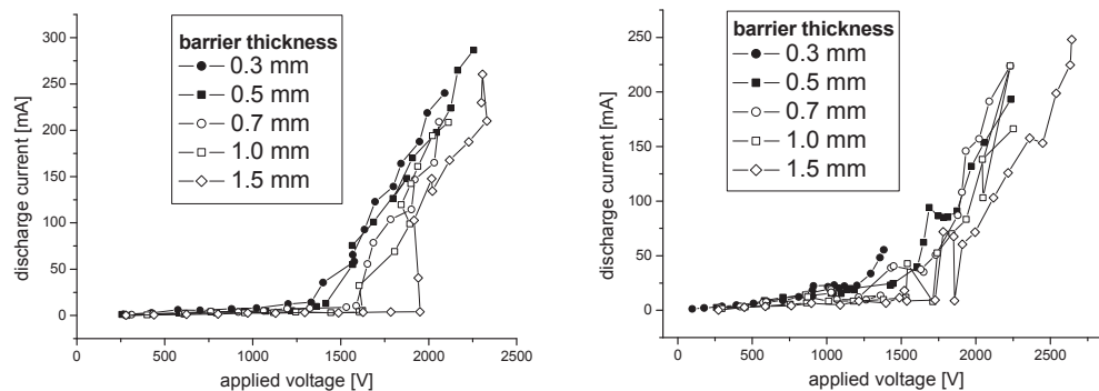
Figure 2. Current-voltage characteristic of the diaphragm discharge breakdown in NaCl solution (250 \mu\text{S}/\text{cm} ). Ceramic diaphragm (orifice of 0.3 mm – left, orifice of 0.6 mm – right), thickness of 0.3–1.5 mm.
