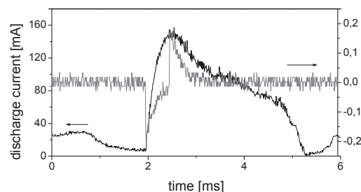
Figure 6. Experiment with the diaphragm with the bigger orifice (diameter of 0.6 mm) and thickness of 1.0 mm. Camera closing by a current impulse (left). Photography exposure time of 0.5 ms (right).
