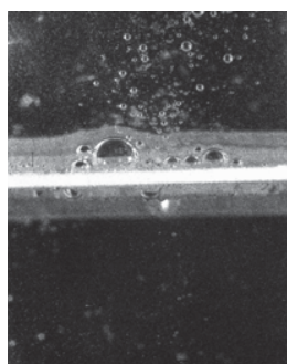
Figure 6. Experiment with the diaphragm with the bigger orifice (diameter of 0.6 mm) and thickness of 1.0 mm. Camera closing by a current impulse (left). Photography exposure time of 0.5 ms (right).
