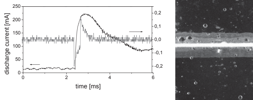
Figure 3. Experiment with the diaphragm with the smaller orifice (diameter of 0.3 mm) and thickness of 0.3 mm. Camera closing by a current impulse (left). Photography exposure time of 0.5 ms (right).
