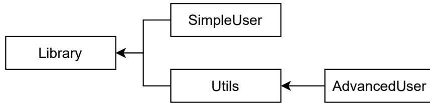
Figure 6.3: The dependency graph between test projects of the end-to-end tests suite.
