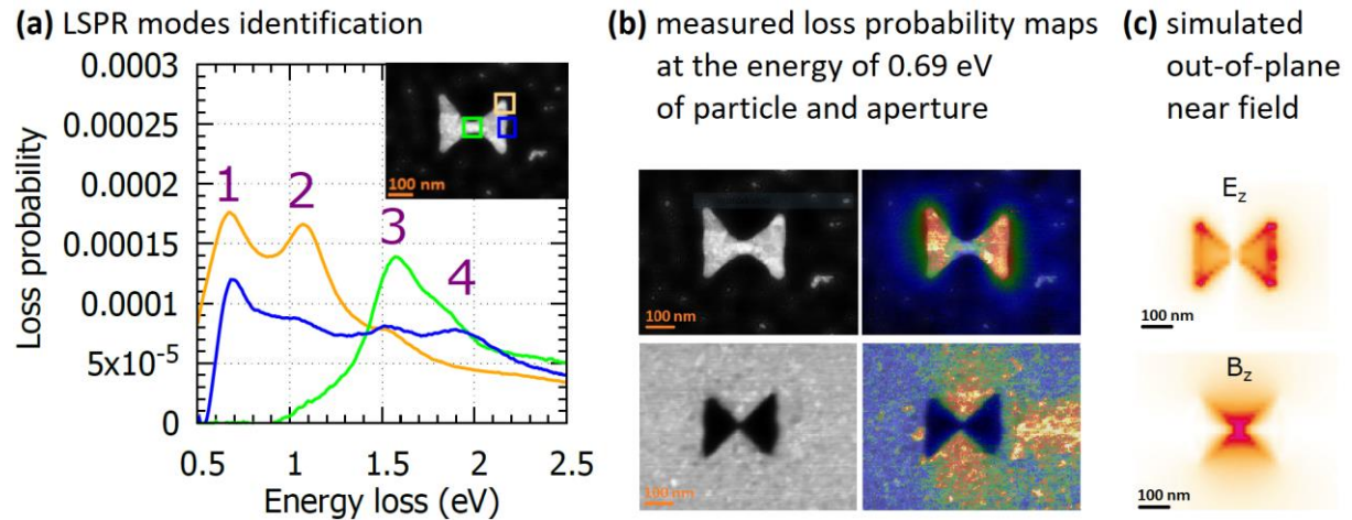
Figure 1: STEM-EELS mapping of the electric and magnetic near field in a diabolo antenna. (a) Identification of four LSPR modes in the diabolo antenna with the total length of 300 nm. (b) STEM annular dark field micrographs of the diabolo (top) and inverted diabolo (bottom) antenna followed by measured loss probability maps at the energy loss of 0.69 eV corresponding to the longitudinal dipole mode for both structures. (c) Calculated electric and magnetic out-of-plane near field distributions for the longitudinal dipole mode in the diabolo antenna.
