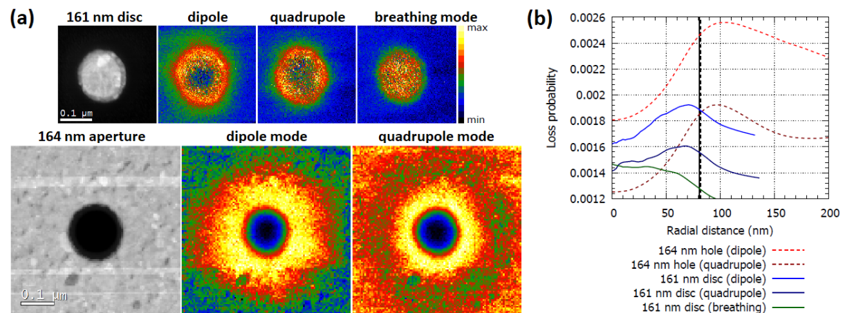
Figure 2: STEM-EELS mapping of the LSPR in a gold disc-shaped plasmonic particle and aperture. (a) STEM annular dark field micrograph of the particle (top) and the aperture (bottom) with measured loss probability maps showing the spatial distribution of LSPR modes: the dipole, quadrupole, and breathing mode. (b) Radial dependency of the loss probability for the LSPR modes.
