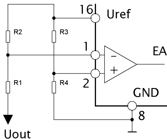
obr. 12 - U_{OUT} < 0 [2]
