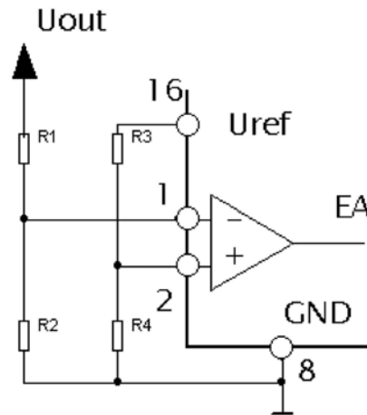
obr. 13 - U_{OUT} > 0 [2]
