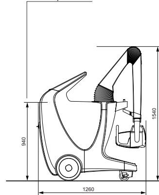
bokorys
