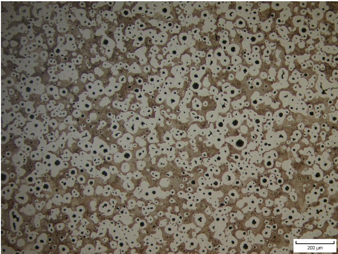
Sample 11T etched, 100x magnification
