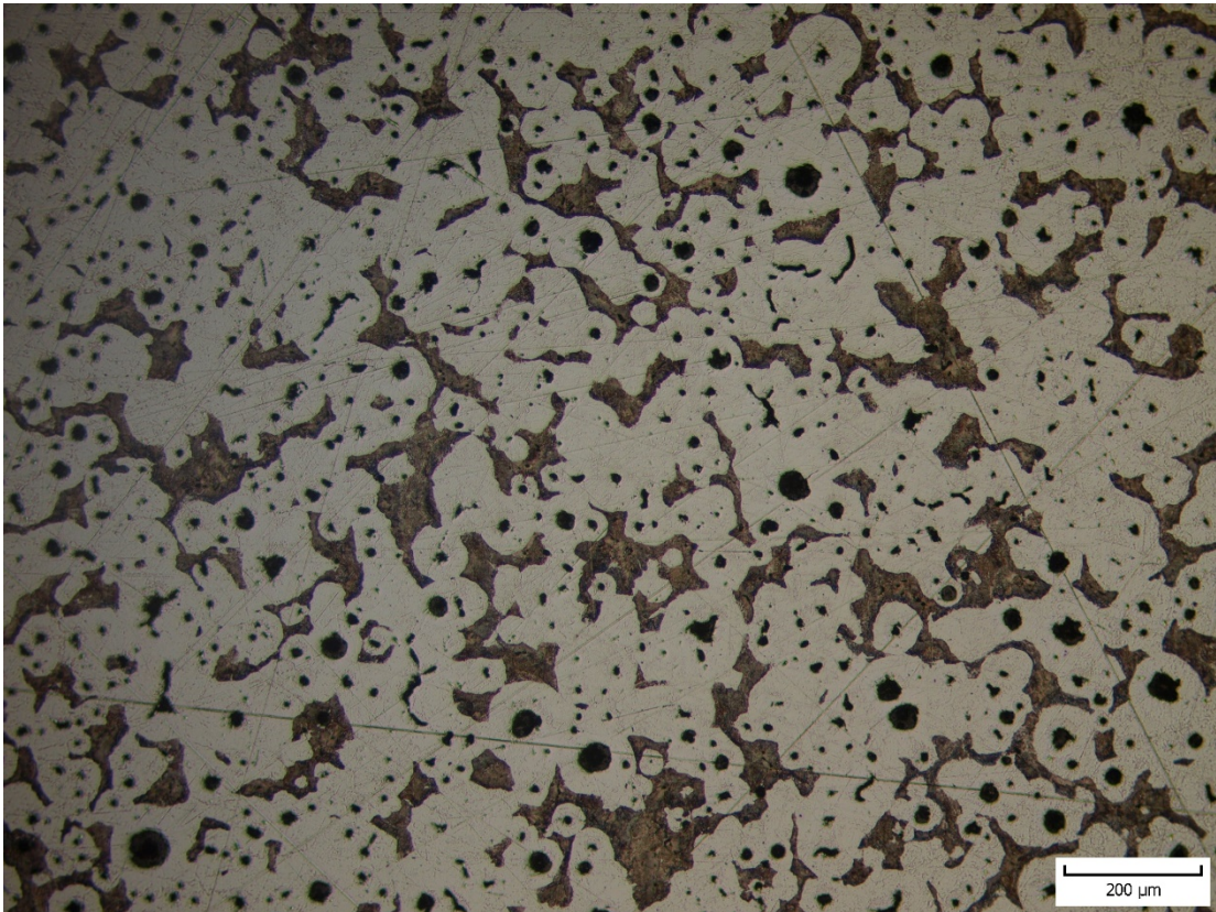
Sample 23 etched, 100x magnification
