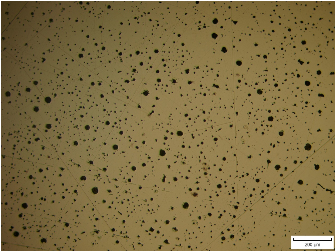
Sample 23T, 100x magnification
