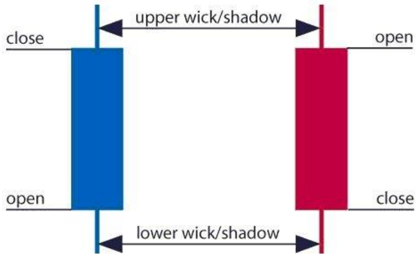
Figure 5: Candlestick bars
