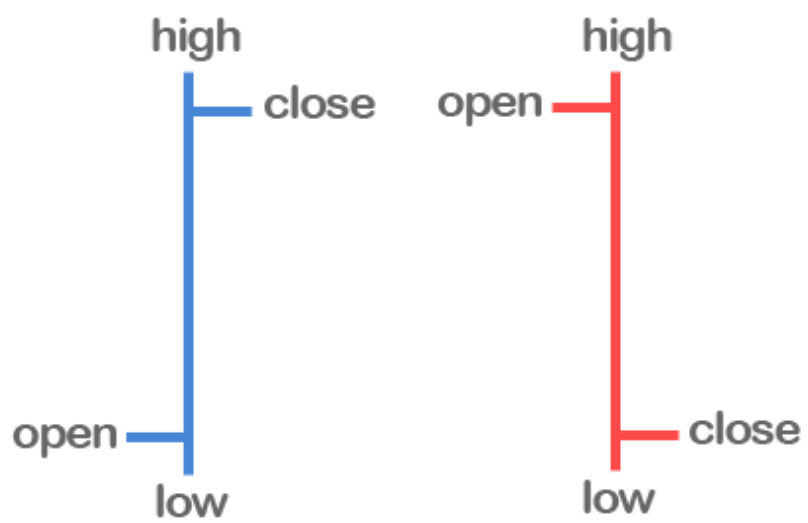
Figure 3: OHLC bars
