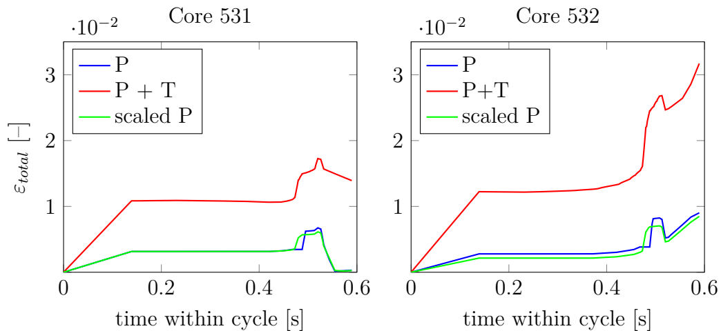
Figure 6.30: Maximum equivalent total strain on the cores during mold filling
