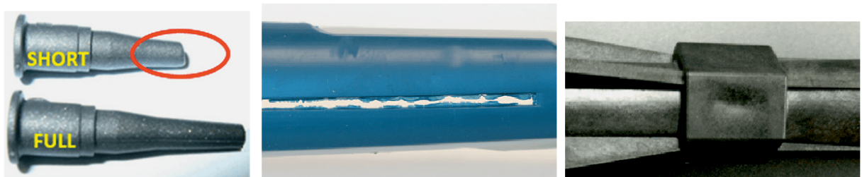
Figure 3.5: From left to right: Short shot, flash and sink marks [5]
