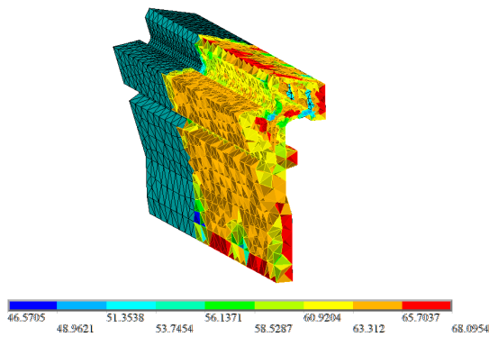
Figure 6.26: Pressures [MPa] from Moldex3D mapped to 532 core mesh
