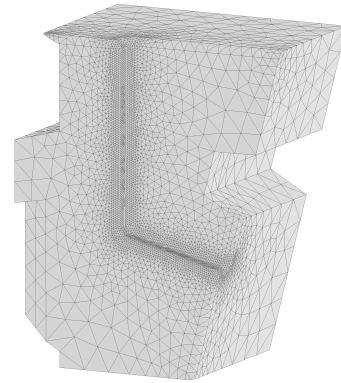
Figure 6.19: Mesh on submodel of core 531
