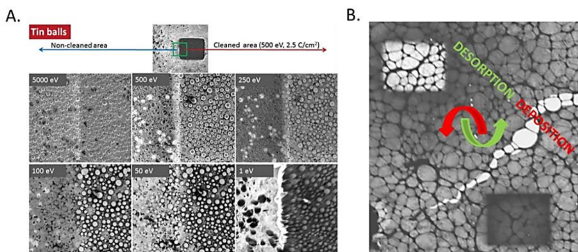
Figure 1 (A) Tin balls observed with 5000 eV, 500 eV, 250 eV, 100 eV, 50 eV, and 1 eV electrons (the left half of each frame shows the non-cleaned area covered with adsorbed molecules, while the right half is the area cleaned by slow electrons); (B) Low voltage STEM observation at 100 eV of graphene after irradiation by electrons that caused deposition (irradiation by 5 keV) and desorption (irradiation by 500 eV).
