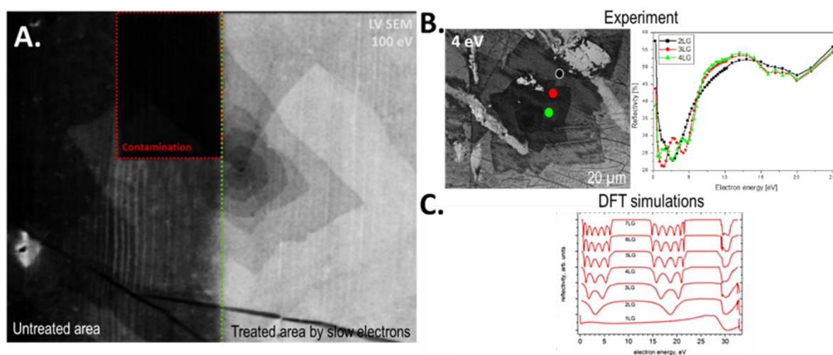
Figure 7 SLEEM study of CVD graphene growth on copper foil (A Multilayered graphene flakes on copper foil: untreated area – treated area by slow electrons – contaminated area by carbon based film after irradiation by higher energy electrons, B Multilayered graphene flakes on copper foil cleaned by slow electrons and measured reflected signal of various thick flakes from 0 eV to 30 eV) supported by DFT simulations (C)
