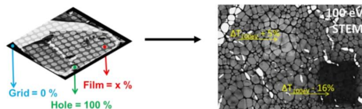
Figure 2 Illustration of the changes in the low-voltage transmissivity of the graphene after electron treatments: cleaning (5% increase)/contamination (16% decrease). The 16-bit image signals were quantified using FIJI software.
