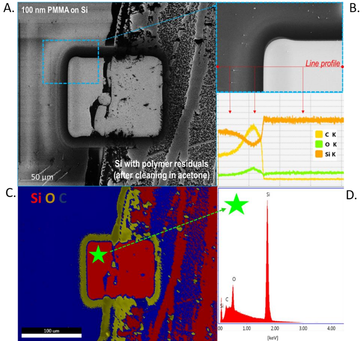
Figure 3 The removal of a 100 nm-thick PMMA by slow electrons (500 eV) observed in SEM (1 keV) and analyze by EDX (A. bright square in the middle of SEM image was irradiated by 500 eV electrons, B. EDX line profile of selected elements: C, O and Si on untreated (dark) and treated (bright) parts, C. EDX mapping of selected area (A) and D. EDX point analysis of cleaned area by slow electrons)
