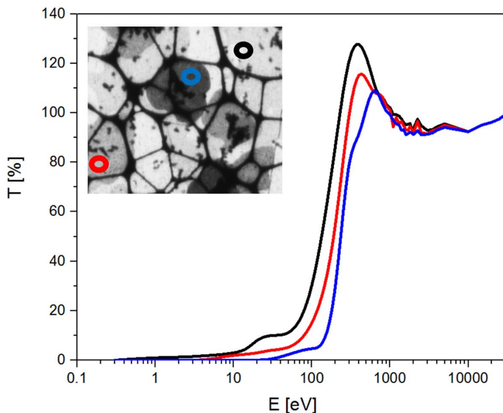
Figure 8 Electron energy dependence of transmissivity from one to several multilayers measured from 30 keV to 0.3 eV.
