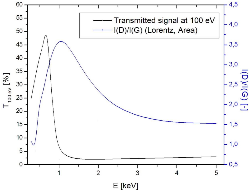
Figure 5 Transmitted signal observed at 100 eV (inserted graphene: 8%) and the intensity ratio of D and G peaks obtained by Raman spectroscopy (inserted sample: 1.5, 300 eV – 1.12, 500 eV – 2.05, 1000 eV – 3.53, 2000 eV – 2.40, 3000 eV – 1.63, 4000 eV – 1.53 and 5000 eV – 1.50) after irradiation as a function of electron-impacted energy
