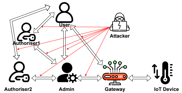
Fig. 2. Threat model.
