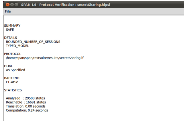
Fig. 12. Protocol status in CL-AtSe.
