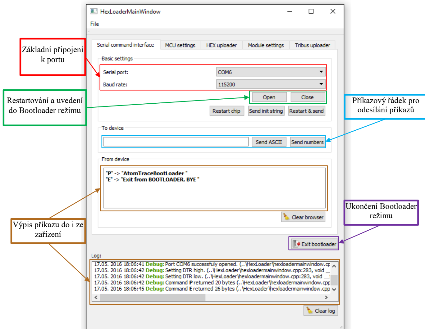
Obr. 21: Popis programu HexLoaderMaster
