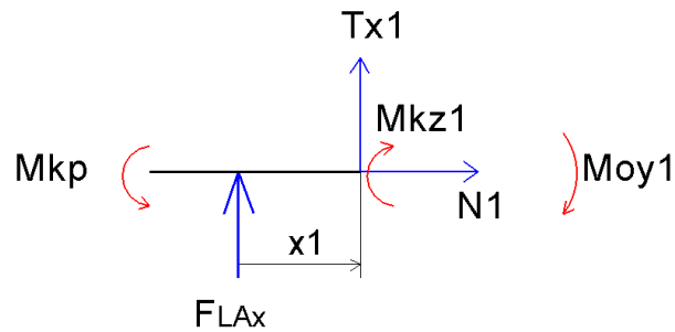
Obr. 35 Interval 1 XZ
