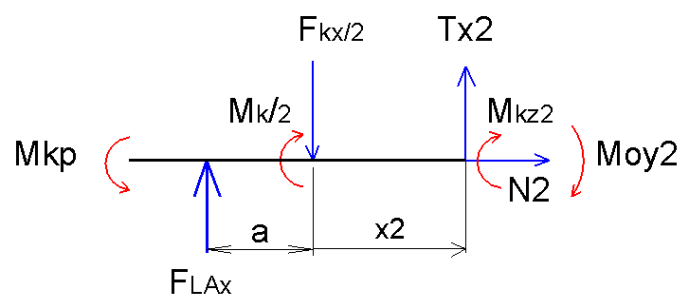
Obr. 36 Interval 2 XZ
