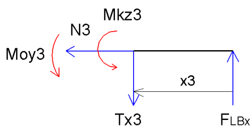
Obr. 37 Interval 3 XZ
