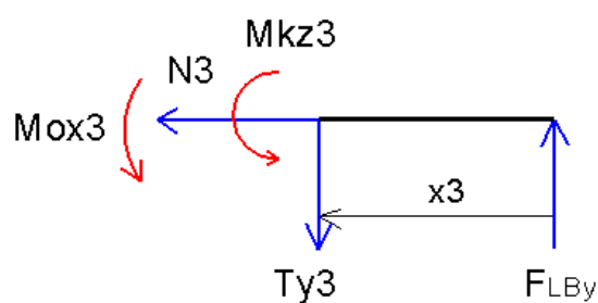
Obr. 32 Interval 3 YZ
