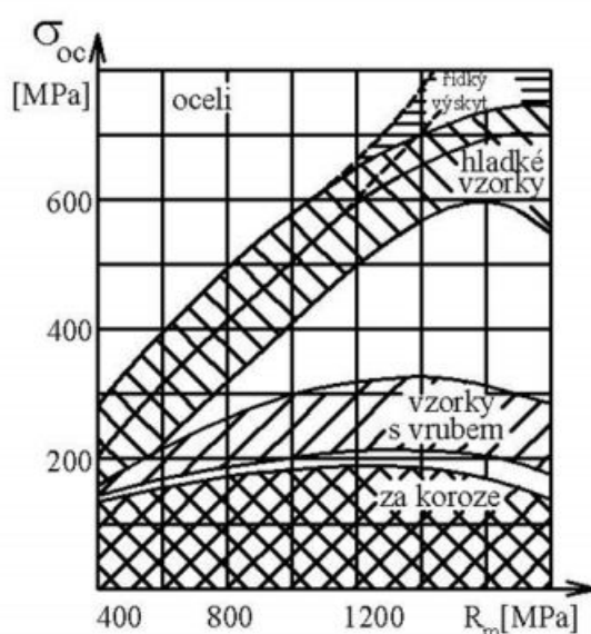
Obr. 40 Mez únavy [16]
