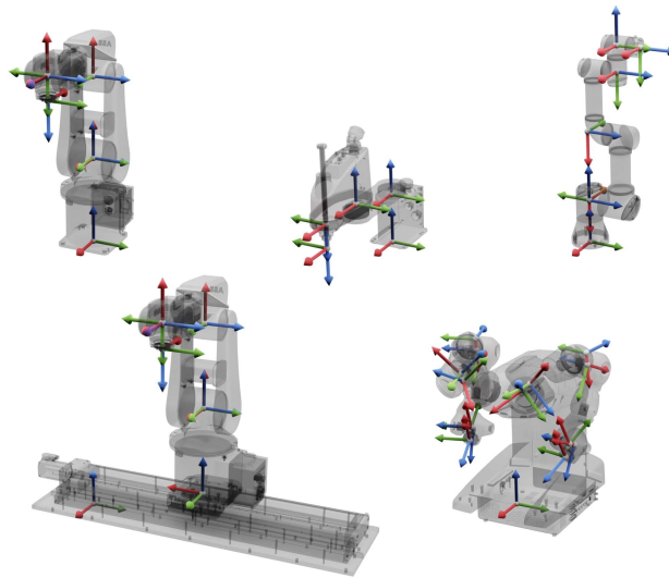
Figure 5.7: An illustration of the geometric representations of the robotic arms portfolio, calculated using the modified Denavit-Hartenberg method.
