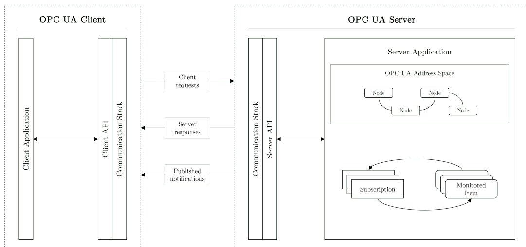
Figure 2.3: Typical client/server architecture of the OPC UA international standard [4].
