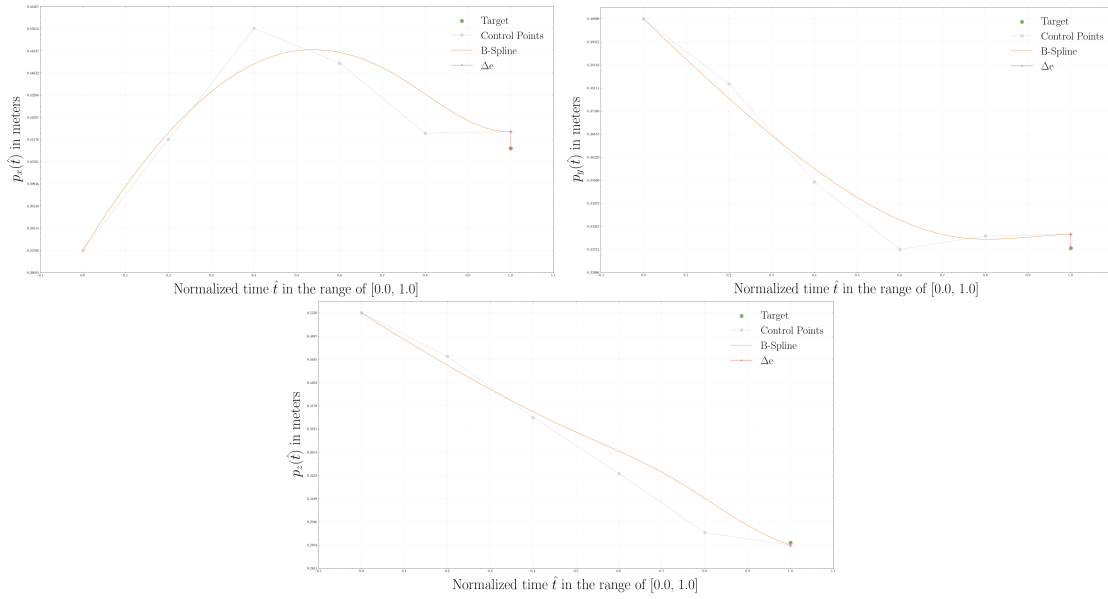
Figure B.3: The results of the positional aspect of the TD3 solution for an environment type \mathcal{E}_1 , interpolated by the parametric B-spline curve of degree n = 3 , regarding the ABB IRB 120 robotic structure extended by a linear axis. The mean absolute error of the predicted solution was equal to e_p = 0.00764 .
