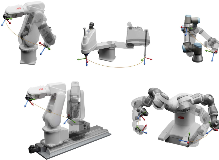
Figure 5.10: An illustration of the kinematic solution trajectory obtained through the informed Levenberg-Marquardt method for an individual robotic structure.
