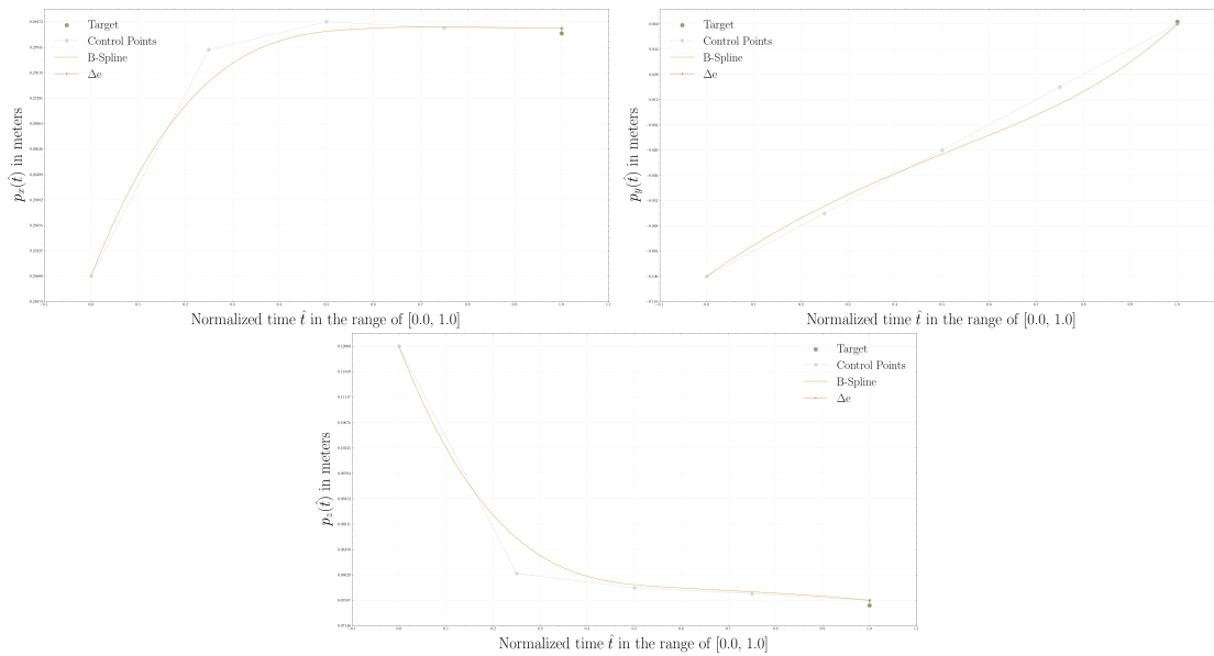
Figure B.12: The results of the positional aspect of the DDPG solution for an environment type \mathcal{E}_2 , interpolated by the parametric B-spline curve of degree n = 3 , regarding the Epson LS3-B401S robotic structure. The mean absolute error of the predicted solution was equal to e_p = 0.00168 .
