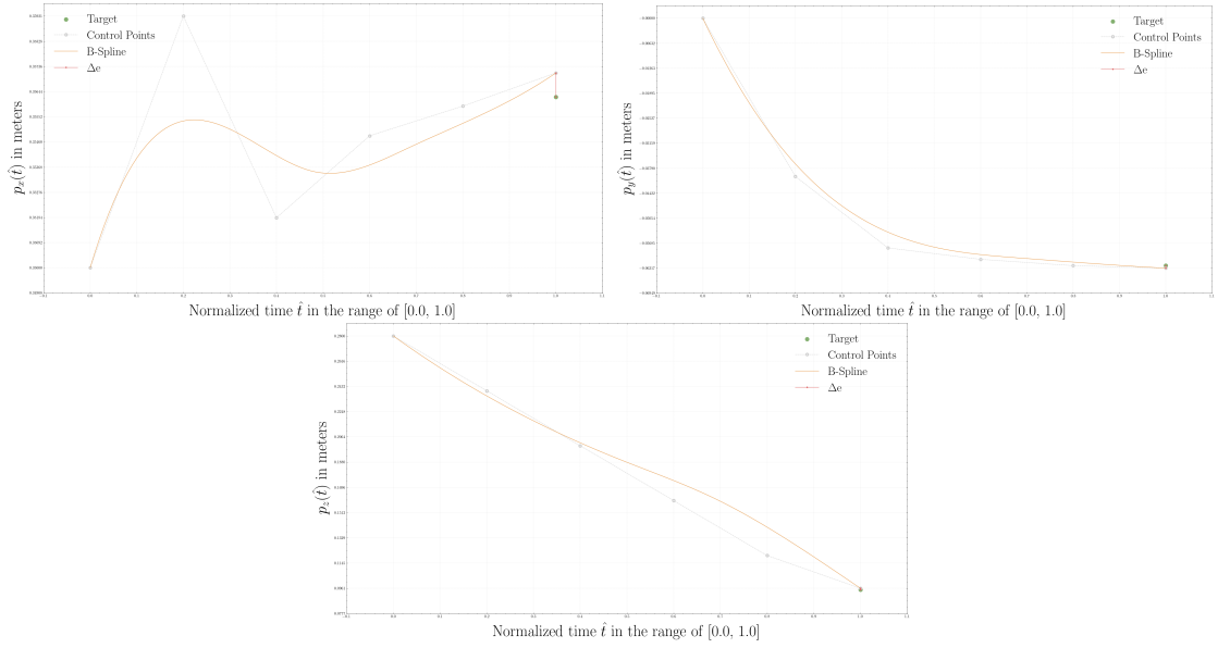
Figure B.1: The results of the positional aspect of the TD3 solution for an environment type \mathcal{E}_1 , interpolated by the parametric B-spline curve of degree n = 3 , regarding the Universal Robots UR3 robotic structure. The mean absolute error of the predicted solution was equal to e_p = 0.00153 .
