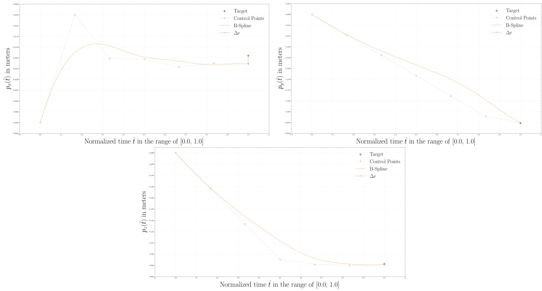
Figure B.10: The results of the positional aspect of the DDPG solution for an environment type \mathcal{E}_2 , interpolated by the parametric B-spline curve of degree n = 3 , regarding the ABB IRB 14000 (left) robotic structure. The mean absolute error of the predicted solution was equal to e_p = 0.00342 .
