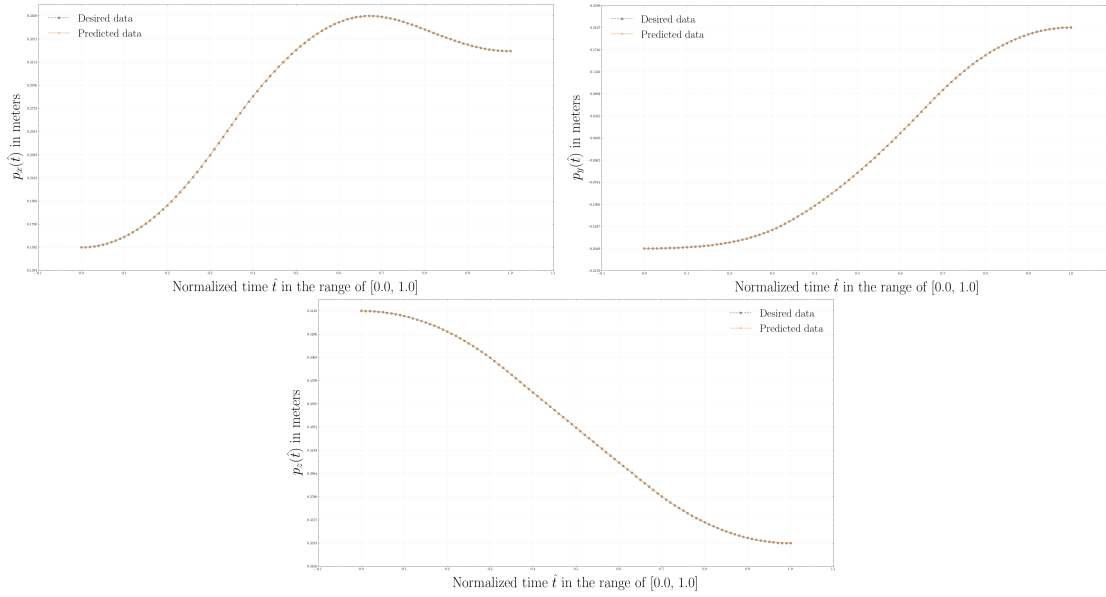
Figure A.4: The results of the positional aspect \mathbf{p} = [p_x, p_y, p_z] of the kinematic solution regarding the ABB IRB 120 robotic structure.
