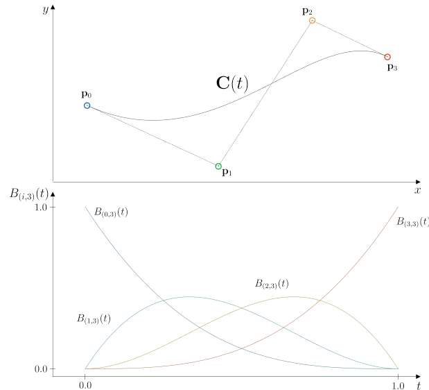
Figure 4.3: A parametric Bézier curve of degree n = 3 (top), denoted as a cubic Bézier curve, with the corresponding representation of Bernstein basis polynomials (bottom).
