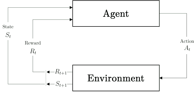
Figure 4.7: The interaction between an agent and the environment in a Markov Decision Process (MDP) [5].
