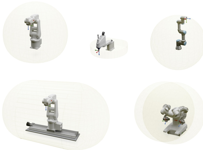
Figure 5.8: An illustration of a simplified version of workspace for the presented robotic arms, determined using the Monte Carlo method.
