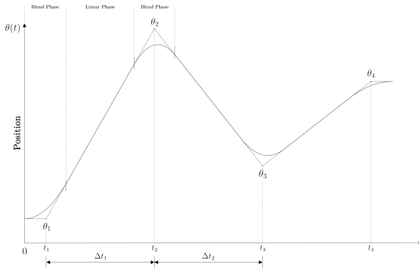
Figure 4.6: Characterization of motion through a sequence of points using a linear function with parabolic blends (LSPB).
