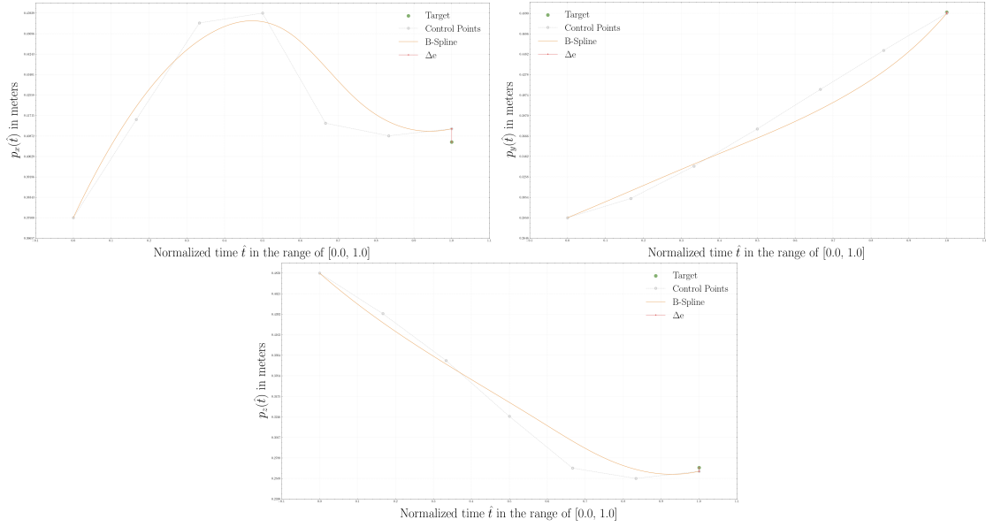
Figure B.9: The results of the positional aspect of the DDPG solution for an environment type \mathcal{E}_2 , interpolated by the parametric B-spline curve of degree n = 3 , regarding the ABB IRB 120 robotic structure extended by a linear axis. The mean absolute error of the predicted solution was equal to e_p = 0.00684 .
