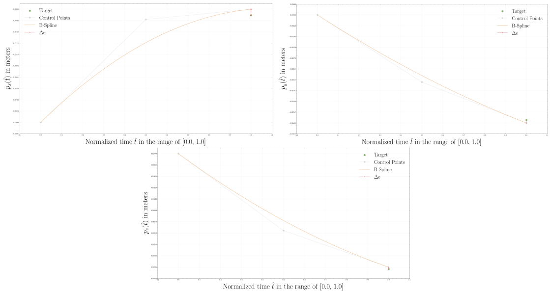
Figure B.6: The results of the positional aspect of the TD3 solution for an environment type \mathcal{E}_1 , interpolated by the parametric B-spline curve of degree n = 2 , regarding the Epson LS3-B401S robotic structure. The mean absolute error of the predicted solution was equal to e_p = 0.00294 .
