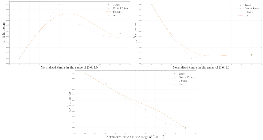
Figure B.2: The results of the positional aspect of the TD3 solution for an environment type \mathcal{E}_1 , interpolated by the parametric B-spline curve of degree n = 3 , regarding the ABB IRB 120 robotic structure. The mean absolute error of the predicted solution was equal to e_p = 0.00750 .
