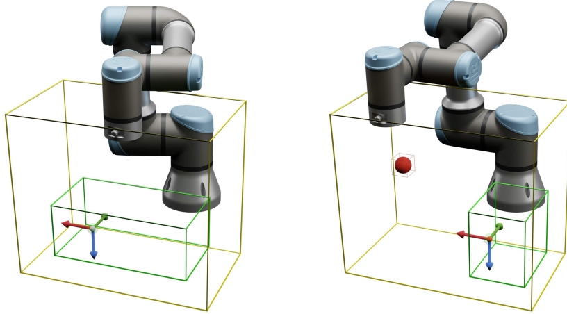
Figure 5.14: An illustration of both types of environments, \mathcal{E}_1 (left) and \mathcal{E}_2 (right), that were used in an experiment focused on reaching the target in a pre-defined configuration space \mathcal{C}_{\text{free}} . The yellow wireframe determines a pre-defined configuration space \mathcal{C}_{\text{free}} , while the green wireframe delineates the area where the target was randomly generated. The red sphere within the environment \mathcal{E}_2 represents an obstacle approximated with AABB, denoted as \mathcal{O}_{\text{AABB}} .
