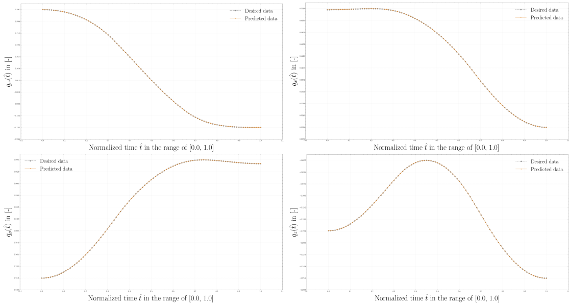
Figure A.7: The results of the orientational aspect \mathbf{Q} = [q_w, q_x, q_y, q_z] of the kinematic solution regarding the ABB IRB 120 robotic structure extended by a linear axis.
