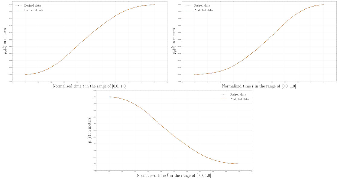
Figure A.6: The results of the positional aspect \mathbf{p} = [p_x, p_y, p_z] of the kinematic solution regarding the ABB IRB 120 robotic structure extended by a linear axis.
