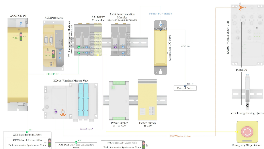
Figure 5.4: The structure of the advanced vertical system integration of the presented robotic workplace.
