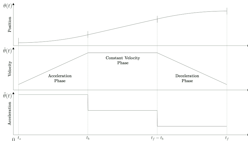
Figure 4.5: Position ( \theta ), velocity ( \dot{\theta} ) and acceleration ( \ddot{\theta} ) of a linear trajectory with a parabola (LSPB), characterized by a trapezoidal motion profile.
