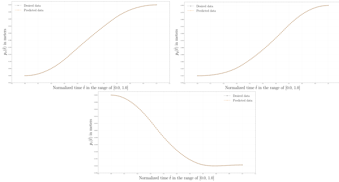
Figure A.12: The results of the positional aspect \mathbf{p} = [p_x, p_y, p_z] of the kinematic solution regarding the ABB IRB 14000 (right) robotic structure.
