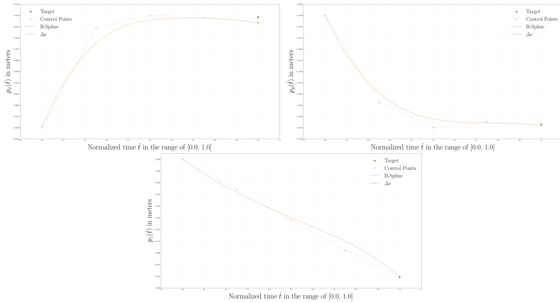
Figure B.4: The results of the positional aspect of the TD3 solution for an environment type \mathcal{E}_1 , interpolated by the parametric B-spline curve of degree n = 3 , regarding the ABB IRB 14000 (left) robotic structure. The mean absolute error of the predicted solution was equal to e_p = 0.00160 .
