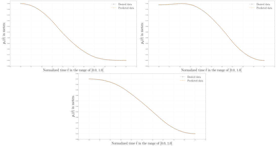
Figure A.2: The results of the positional aspect \mathbf{p} = [p_x, p_y, p_z] of the kinematic solution regarding the Universal Robots UR3 robotic structure.
