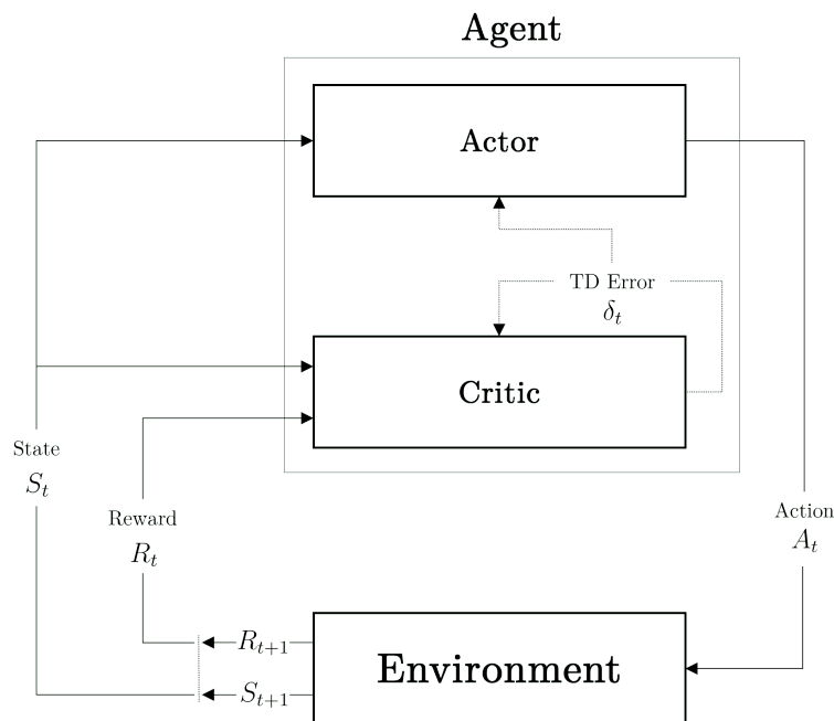
Figure 4.8: An overview of the actor-critic architecture. The Temporal Difference (TD) error \delta_t is utilized to adjust both the critic’s action value function Q(s, a) and the actor’s policy \pi(a | s, \theta) , which is parameterized by \theta [5, 6].
