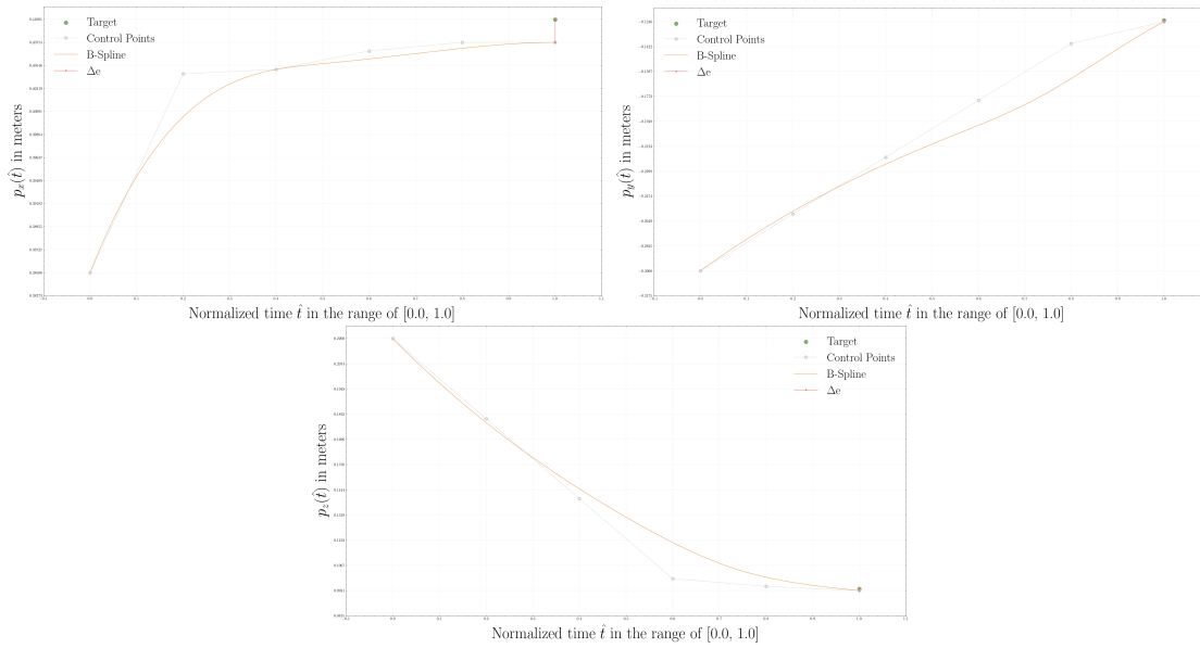
Figure B.11: The results of the positional aspect of the DDPG solution for an environment type \mathcal{E}_2 , interpolated by the parametric B-spline curve of degree n = 3 , regarding the ABB IRB 14000 (right) robotic structure. The mean absolute error of the predicted solution was equal to e_p = 0.00260 .
