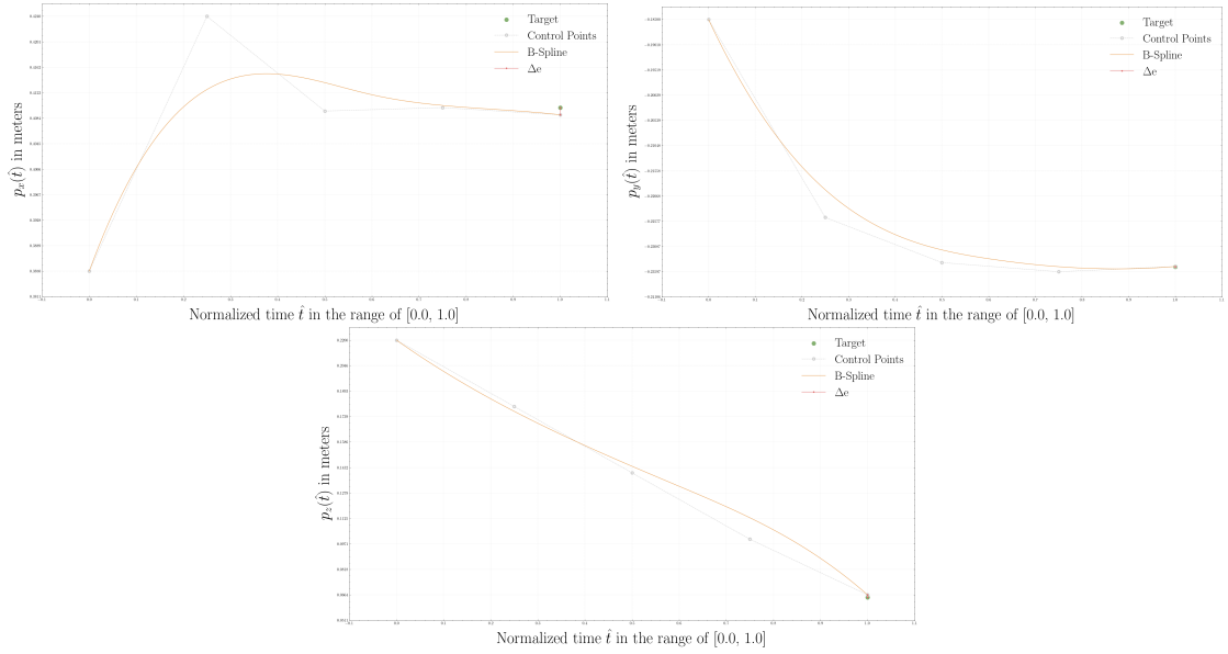
Figure B.5: The results of the positional aspect of the TD3 solution for an environment type \mathcal{E}_1 , interpolated by the parametric B-spline curve of degree n = 3 , regarding the ABB IRB 14000 (right) robotic structure. The mean absolute error of the predicted solution was equal to e_p = 0.00179 .
