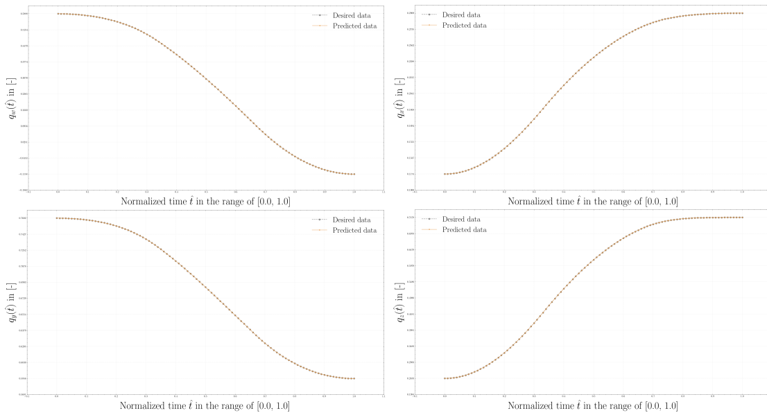
Figure A.13: The results of the orientational aspect \mathbf{Q} = [q_w, q_x, q_y, q_z] of the kinematic solution regarding the ABB IRB 14000 (right) robotic structure.
