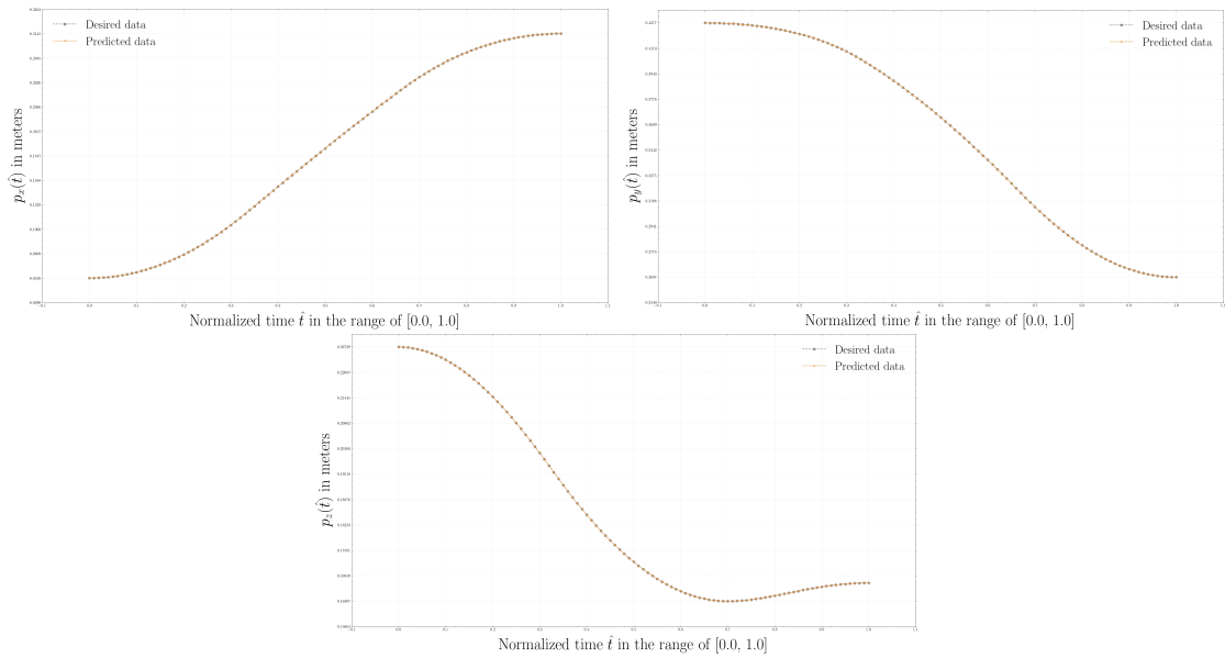
Figure A.10: The results of the positional aspect \mathbf{p} = [p_x, p_y, p_z] of the kinematic solution regarding the ABB IRB 14000 (left) robotic structure.
