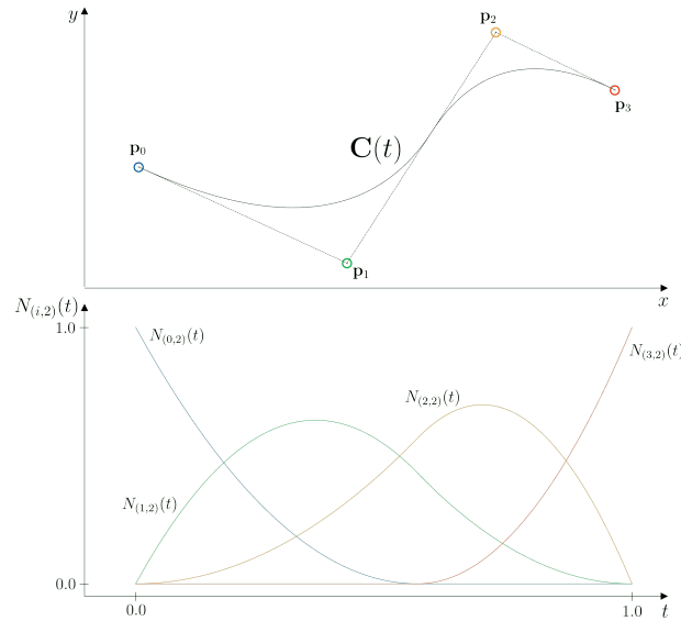
Figure 4.4: A parametric B-spline curve of degree n = 2 (top), with the corresponding representation of B-Spline basis functions (bottom).
