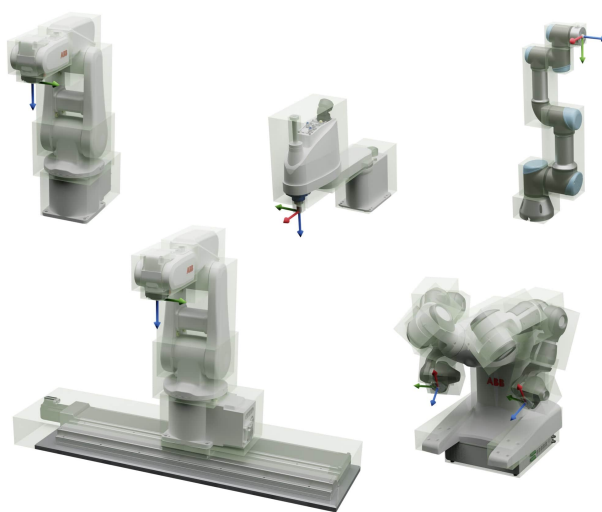
Figure 5.9: An illustration of the collision structures of the robotic arm portfolio, represented using Oriented Bounding Boxes (OBBs).
