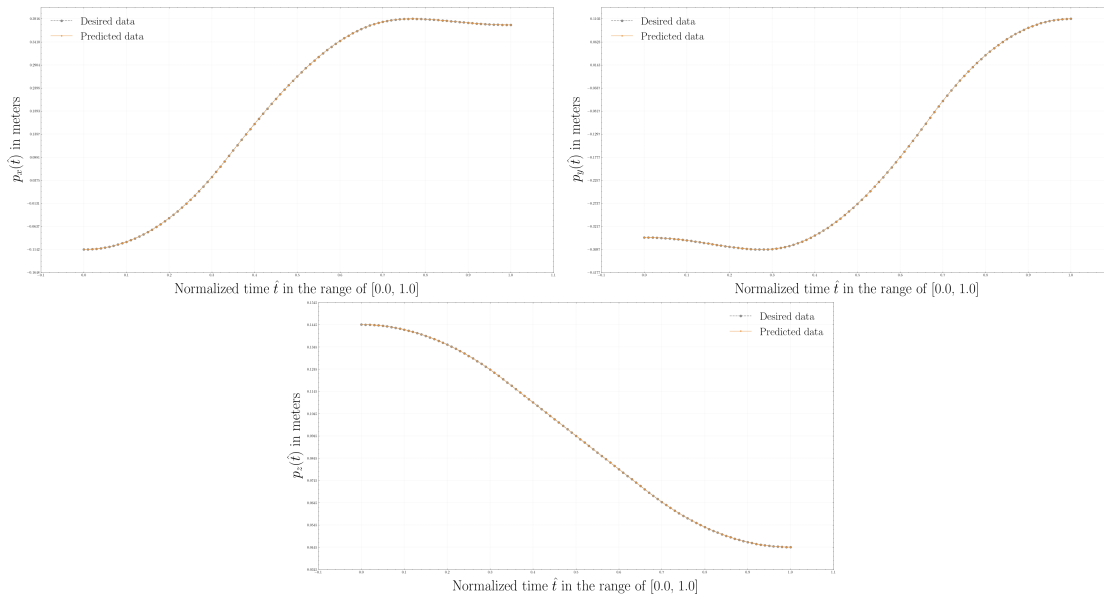
Figure A.8: The results of the positional aspect \mathbf{p} = [p_x, p_y, p_z] of the kinematic solution regarding the Epson LS3-B401S robotic structure.
