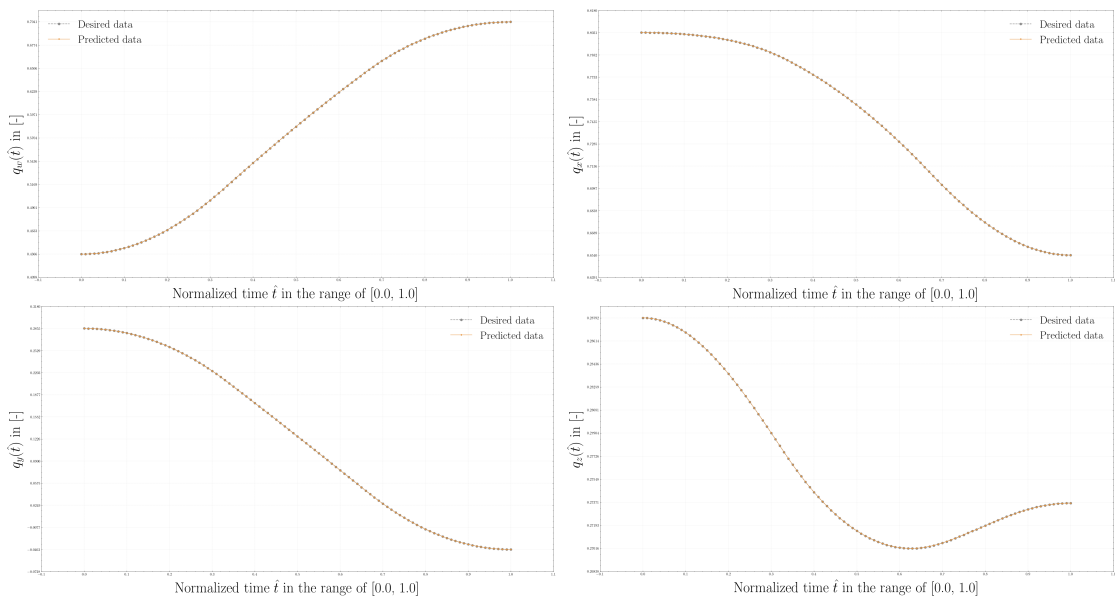
Figure A.11: The results of the orientational aspect \mathbf{Q} = [q_w, q_x, q_y, q_z] of the kinematic solution regarding the ABB IRB 14000 (left) robotic structure.
