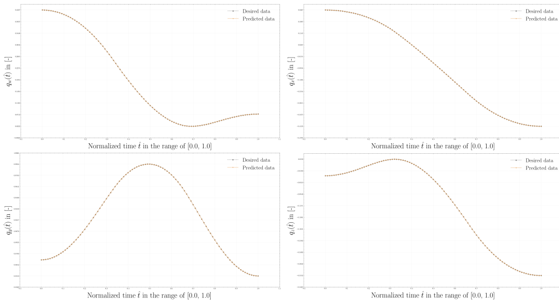
Figure A.5: The results of the orientational aspect \mathbf{Q} = [q_w, q_x, q_y, q_z] of the kinematic solution regarding the ABB IRB 120 robotic structure.
