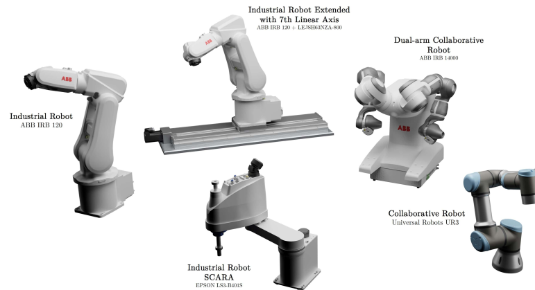
Figure 5.1: An illustration of the robotic structures that are part of the Industry 4.0 Cell (I4C).
