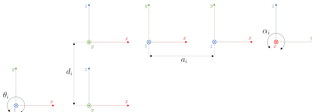
Figure 3.4: Illustration of the Denavit-Hartenberg convention defined by the four parameters a_i , \alpha_i , d_i , and \theta_i .
