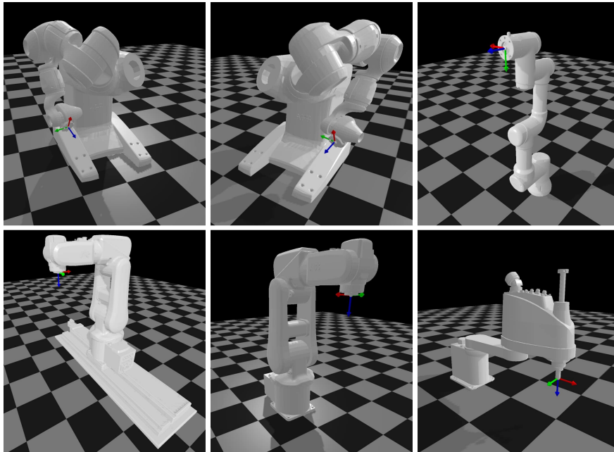
Figure A.1: An illustration of the various robotic structures used to test the kinematic solution. In the top row, there are the right and left arms of the ABB IRB 14000 and the Universal Robots UR3. In the bottom row, there is an ABB IRB 120 extended by a linear axis, the same robot without an extension, and lastly, the Epson LS3-B401S.
