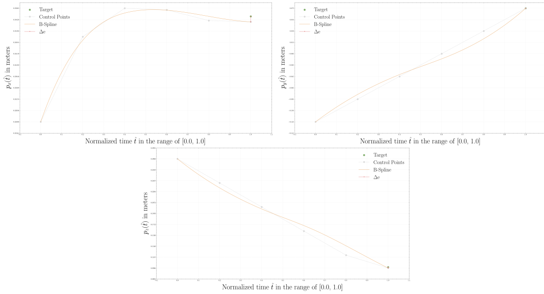
Figure B.7: The results of the positional aspect of the DDPG solution for an environment type \mathcal{E}_2 , interpolated by the parametric B-spline curve of degree n = 3 , regarding the Universal Robots UR3 robotic structure. The mean absolute error of the predicted solution was equal to e_p = 0.00215 .
