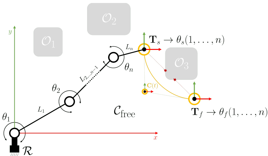
Figure 4.1: A schematic representation of a motion planning problem in two-dimensional space, illustrating an n -link robotic manipulator \mathcal{R} within a collision-free configuration space \mathcal{C}_{\text{free}} with obstacles denoted as \mathcal{O} .
