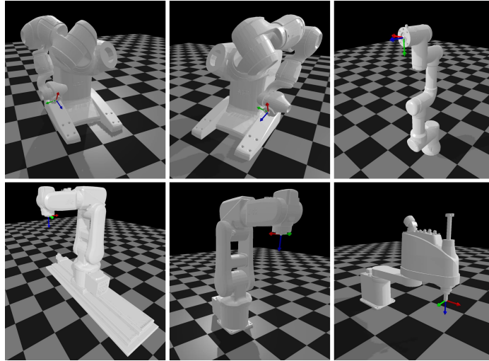
Figure 5.11: An illustration of the robotic structures that are part of the Industry 4.0 Cell (I4C) within the PyBullet physical simulation.
