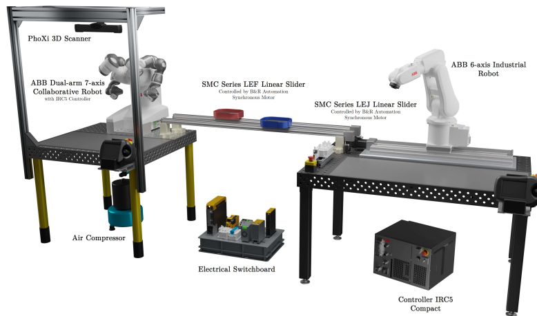
Figure 5.2: The fundamental concept of the Versatile Intelligent Robotic Workstation (VInRoS), which illustrates its main components.
