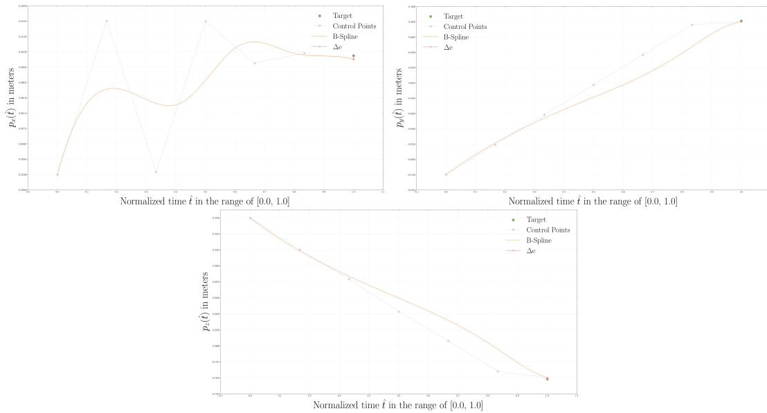
Figure B.8: The results of the positional aspect of the DDPG solution for an environment type \mathcal{E}_2 , interpolated by the parametric B-spline curve of degree n = 3 , regarding the ABB IRB 120 robotic structure. The mean absolute error of the predicted solution was equal to e_p = 0.00184 .
