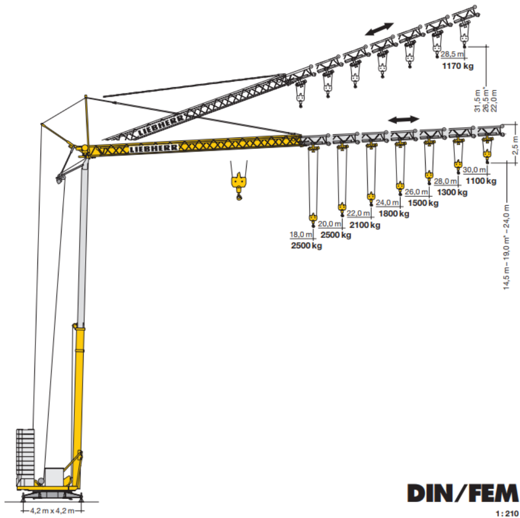
Obr. 12.3 Liebherr 32TT
