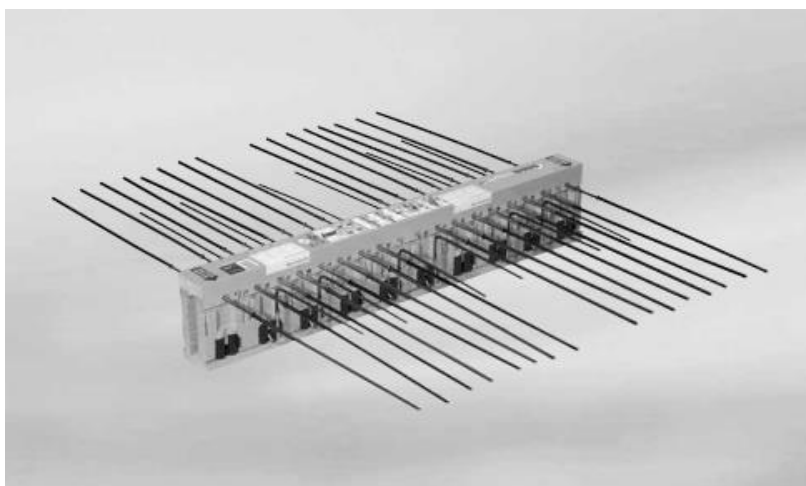
Obr. 4.27 Isokorb K50S-CV30-V8
