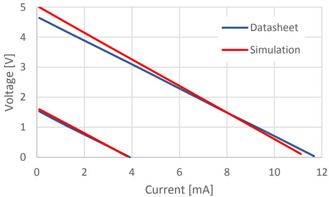
Fig. 19 Voltage vs. current curves for \Delta T=10\text{ }^{\circ}\text{C} and \Delta T=30\text{ }^{\circ}\text{C}
