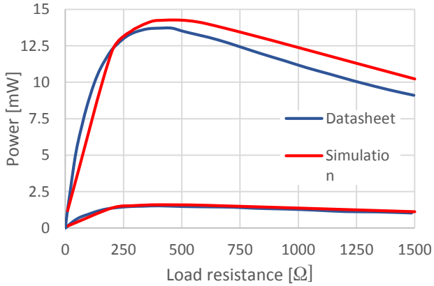
Fig. 18 Power vs. load resistance for \Delta T=10\text{ }^{\circ}\text{C} and \Delta T=30\text{ }^{\circ}\text{C}
