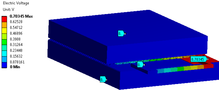
Fig. 15 Voltage distribution in the MPG-D751
