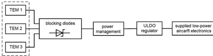
Fig. 20 System block diagram of TEG power source for aircraft application
