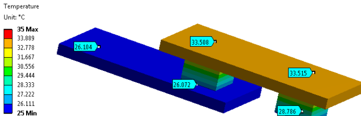
Fig. 14 Temperature distribution in the thermocouple
