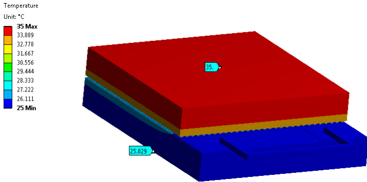
Fig. 13 Temperature distribution in module MPG-D751
