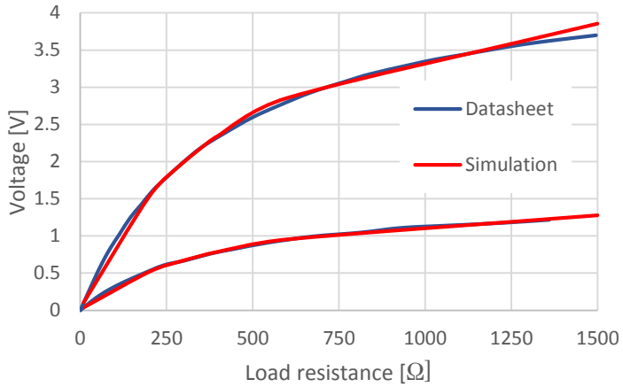
Fig. 17 Voltage vs. load resistance for \Delta T=10\text{ }^\circ\text{C} and \Delta T=30\text{ }^\circ\text{C}
