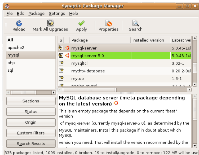
Obr. 3.4: MySQL-server5.
