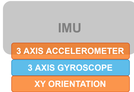
Figure 5.10: IMU Design Requirements Block
