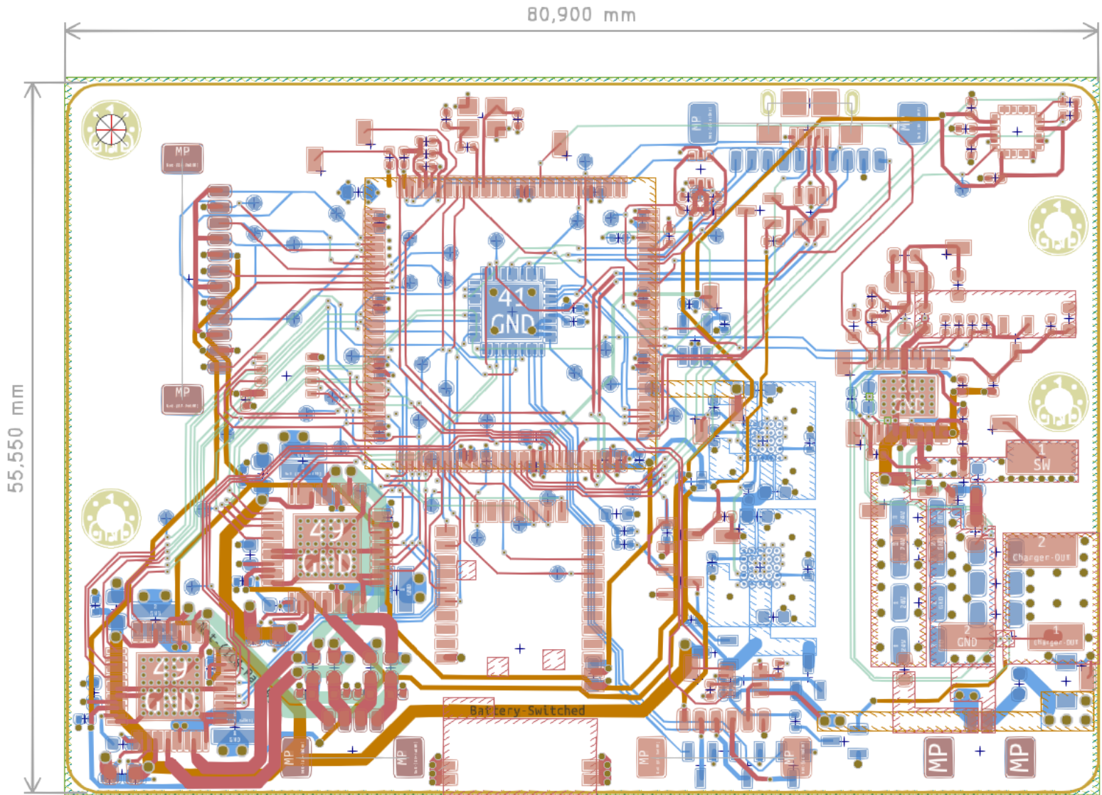
Figure 5.27: PCB Schematic, 6 Layers, Components on Both Sides. Note: Schematics of individual layers can be found in the appendixes 17 to 22
