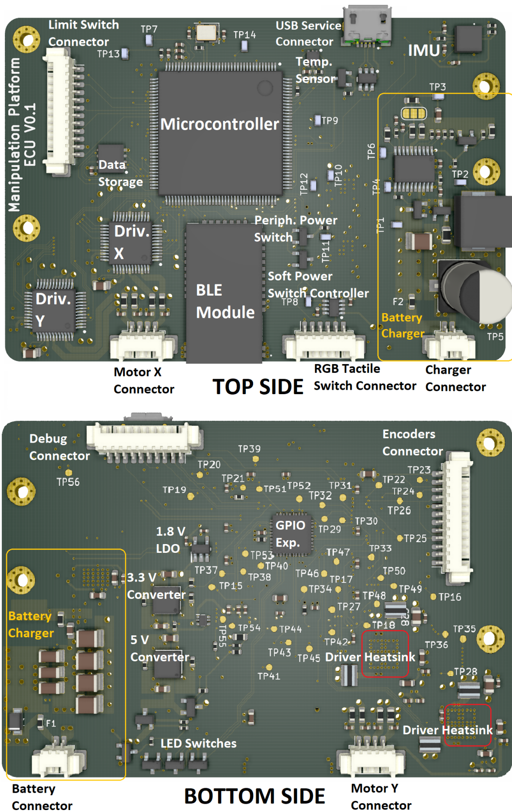
Figure 5.28: Labelled 3D Model of the ECU Printed Circuit Board.
