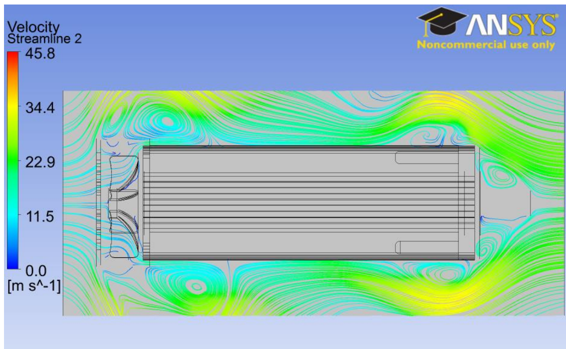
Fig. 5.9: Velocity streamlines along a longitudinal-section of the servo motor with external cooling.
