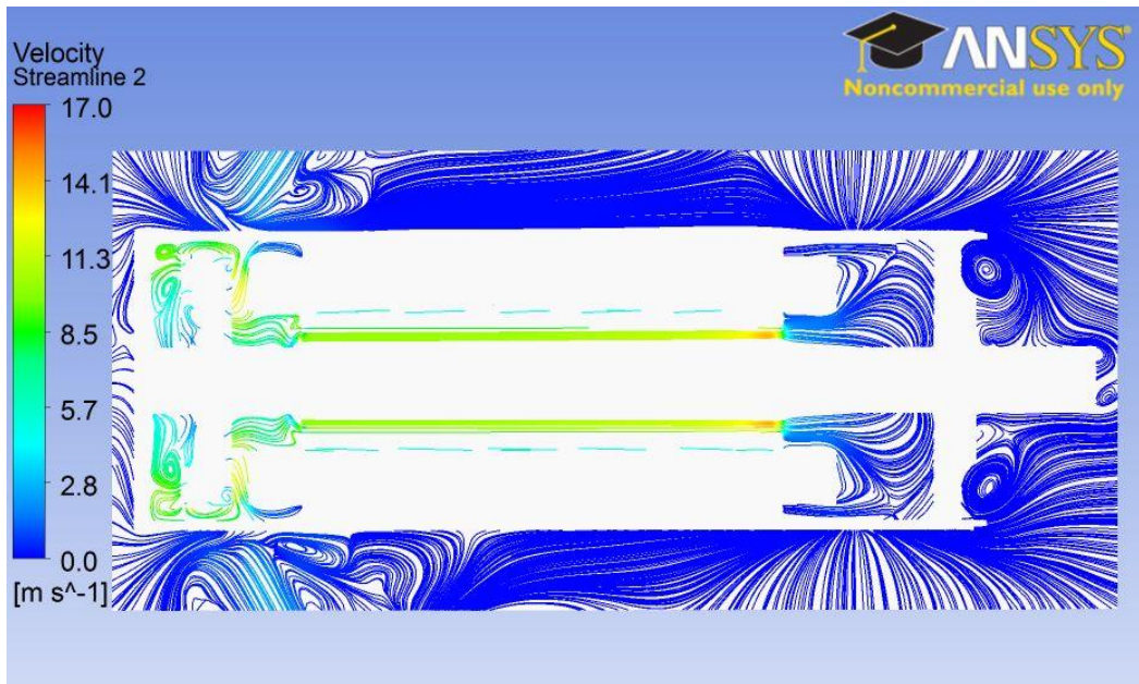
Fig. 5.3: Velocity streamlines along a longitudinal-section of the modified servo motor.
