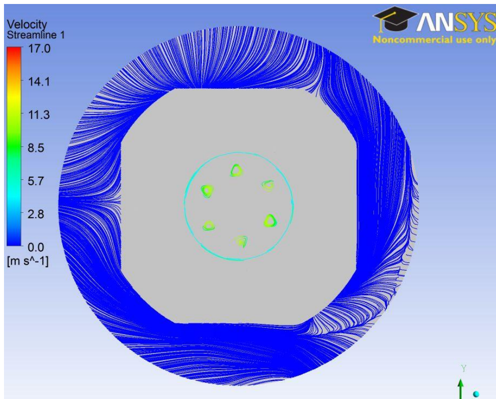
Fig. 5.2: Velocity streamlines along a cross-section of the modified servo motor.
