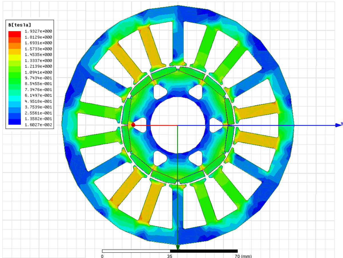
Fig. 3.3: Distribution of magnetic flux density along a cross-section of the servo motor.
