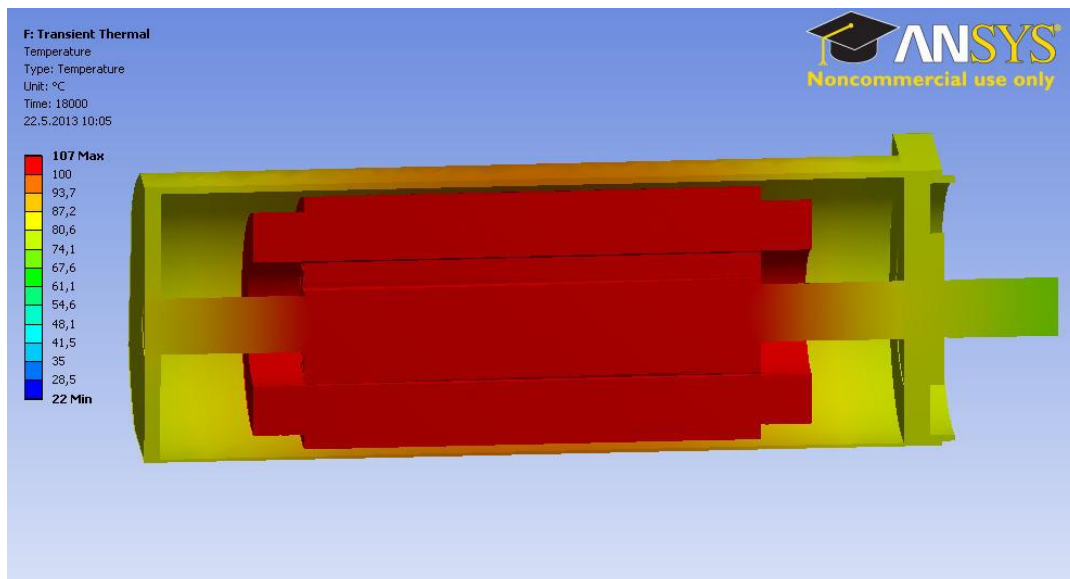
Fig. 5.4: Distribution of temperature field for the original servo motor.
