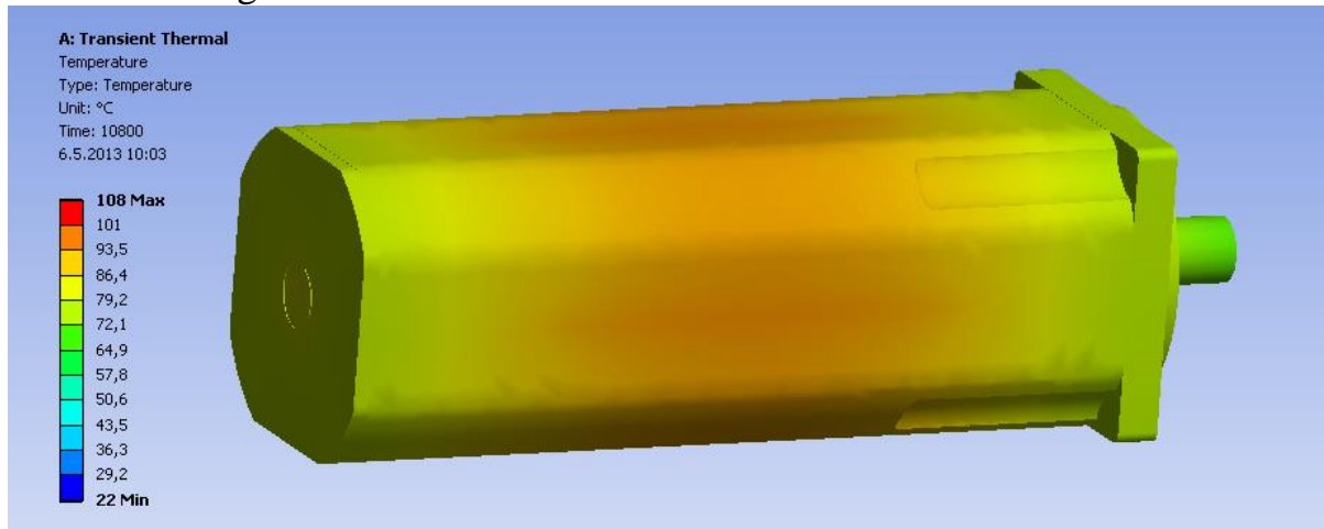
Fig. 5.10: Distribution of temperature field for the original servo motor.
