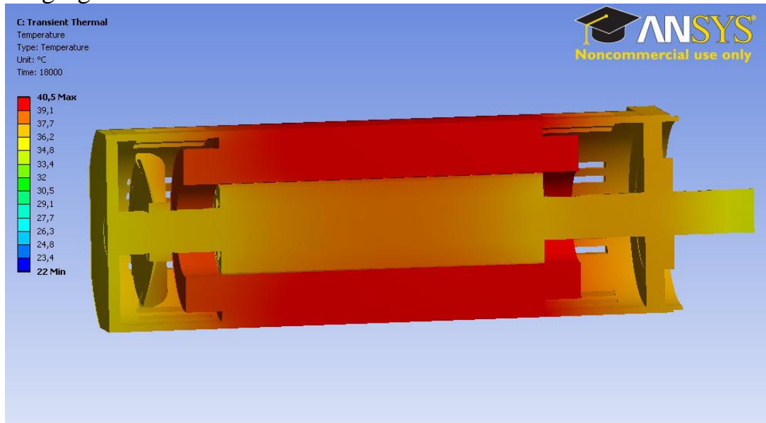
Fig. 5.5: Distribution of temperature field for the modified servo motor.
