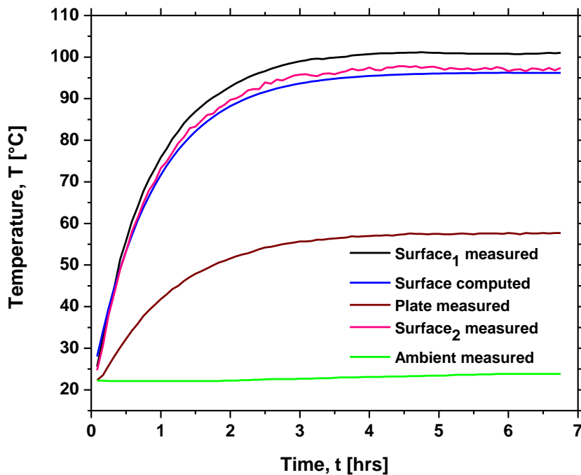
Fig. 6.3: Comparison of measured and computed temperature at surface of the servo motor (surface 1 is surface on top, surface 2 is surface on side).
